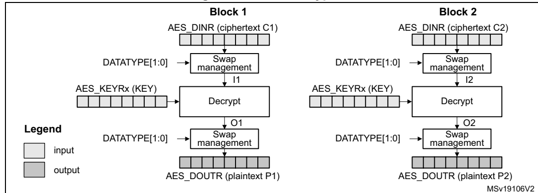
Figure 75. ECB decryption
