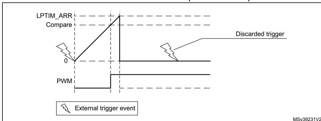
Figure 186. LPTIM output waveform, Single counting mode configuration and Set-once mode activated (WAVE bit is set)
