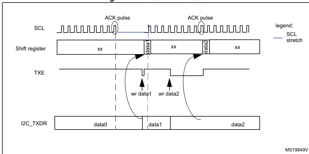
Figure 200. Data transmission
