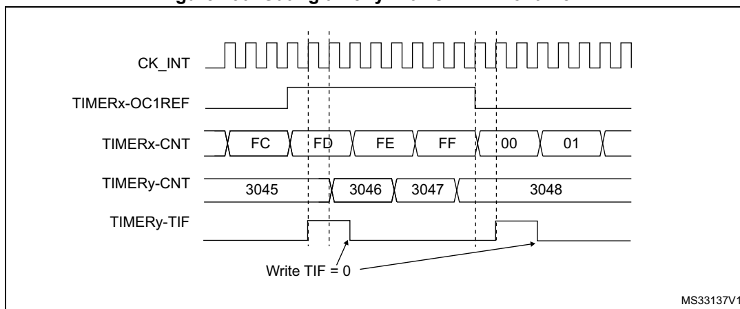
Figure 130. Gating timer y with OC1REF of timer x
