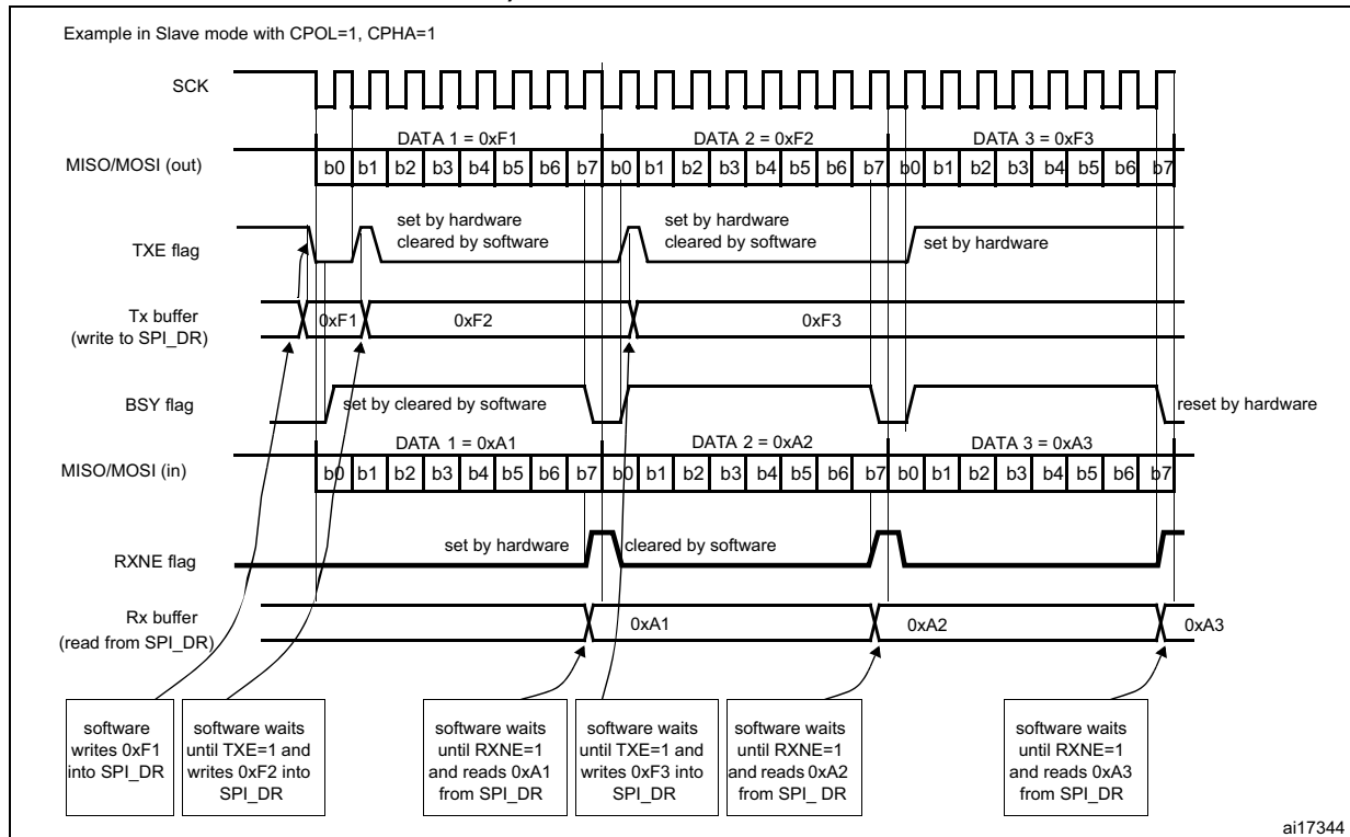
Figure 272. TXE/RXNE/BSY behavior in slave / full-duplex mode (BIDIMODE=0, RXONLY=0) in the case of continuous transfers
