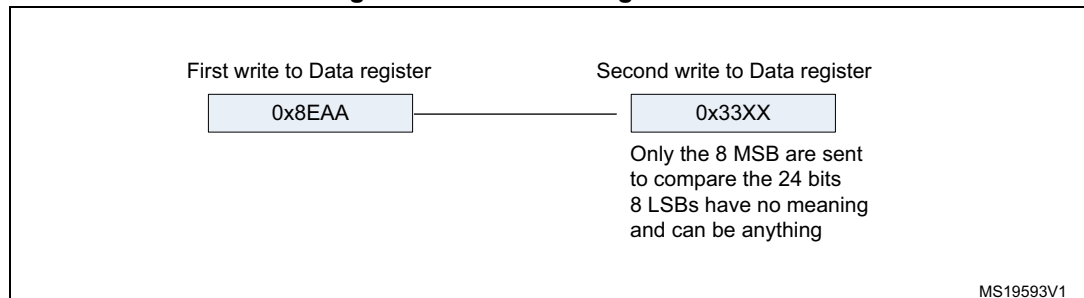
Figure 280. Transmitting 0x8EAA33
