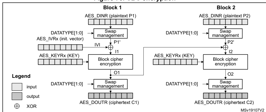
Figure 76. CBC encryption
