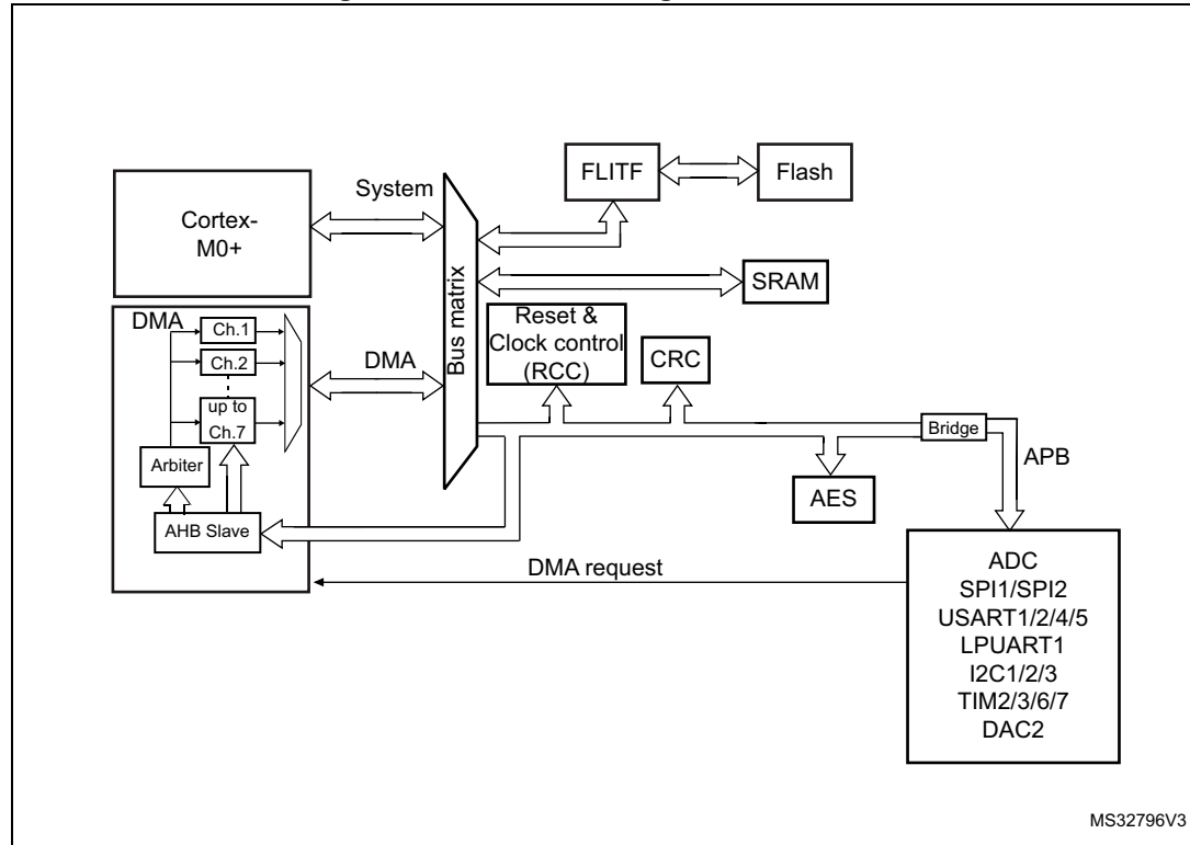
Figure 27. DMA block diagram
