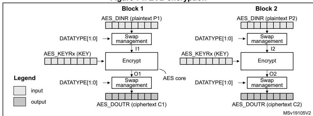
Figure 74. ECB encryption
