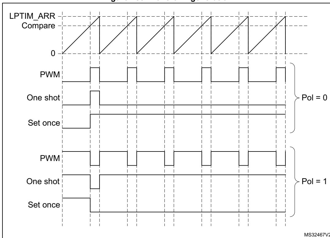
Figure 188. Waveform generation
