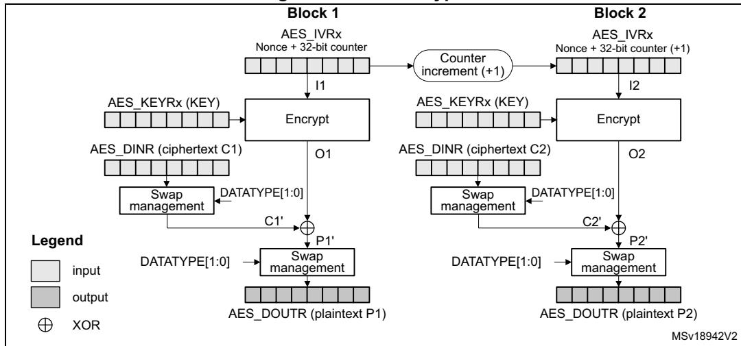
Figure 82. CTR decryption
