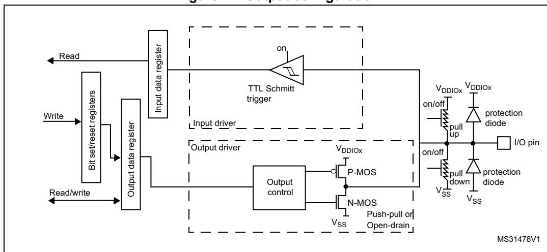
Figure 24. Output configuration
