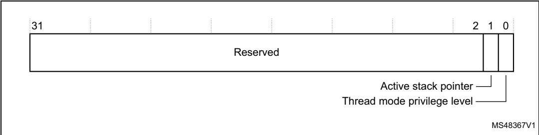
Figure 8. CONTROL bit assignments
