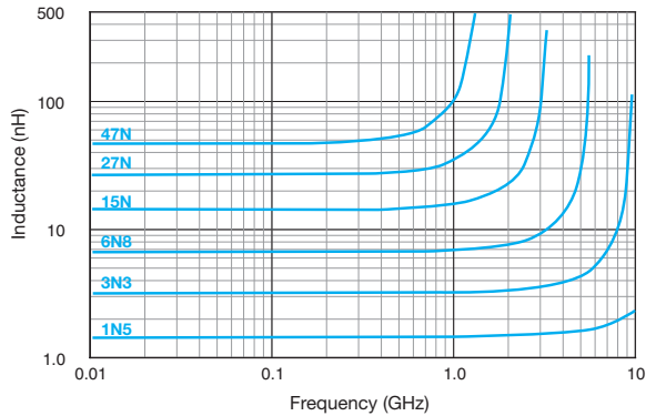
INDUCTANCE VS FREQUENCY: SIZE 0603
