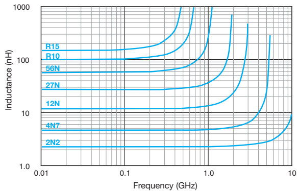
INDUCTANCE VS FREQUENCY: SIZE 0805
