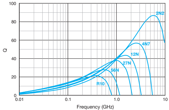
Q VS FREQUENCY: SIZE 0805
