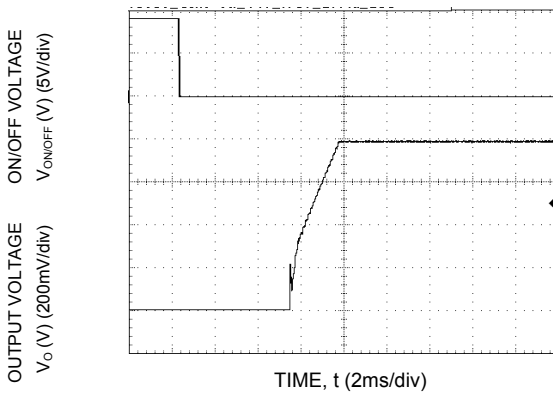
Figure 3. Typical Start-up Using On/Off Voltage ( I_o = I_{o,max} ).
