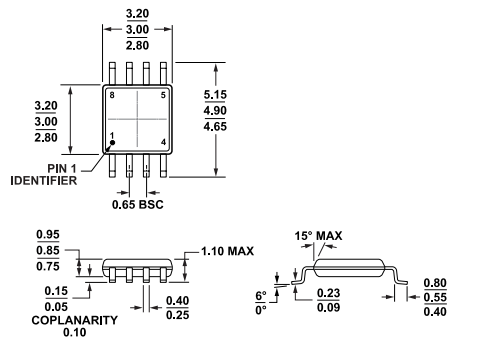
Figure 49. 8-Lead Mini Small Outline Package [MSOP] (RM-8)
