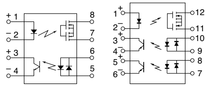
Relay portion (1,2,7,8 pins)
