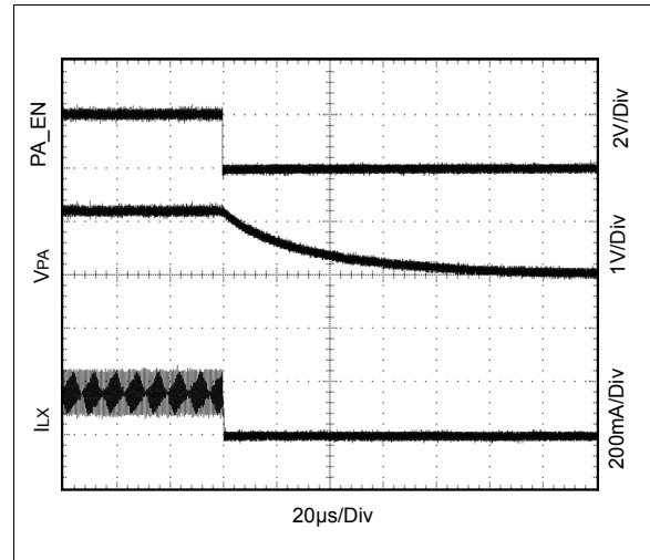
Figure 34. DC-DC Shutdown
