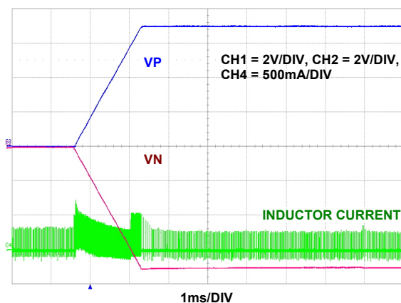
FIGURE 65. VP AND VN ( \pm 7\text{V} ) SOFT-START AT 2.5V INPUT VOLTAGE, VP/VN START TOGETHER (Reg 0x04 \langle b_4 \rangle = 1 )
