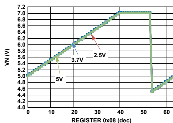
FIGURE 9. V_N OUTPUT VOLTAGE RANGE
