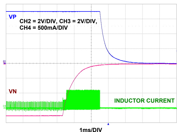
FIGURE 64. VP AND VN ( \pm 7\text{V} ) SHUTDOWN, VP/VN SEQUENCED (Reg 0x05 \langle b_4 \rangle = 0 )
