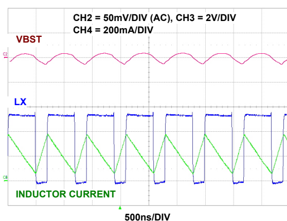
FIGURE 15. VBST RIPPLE, 150mA LOAD, VBST = 5.15V
