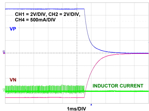
FIGURE 68. VP AND VN ( \pm 7\text{V} ) SHUTDOWN, VP/VN SHUTDOWN TOGETHER (Reg 0x05 \langle b_4 \rangle = 1 )
