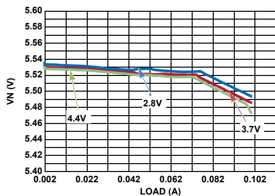
FIGURE 70. VN LOAD REGULATION, -5.5V
