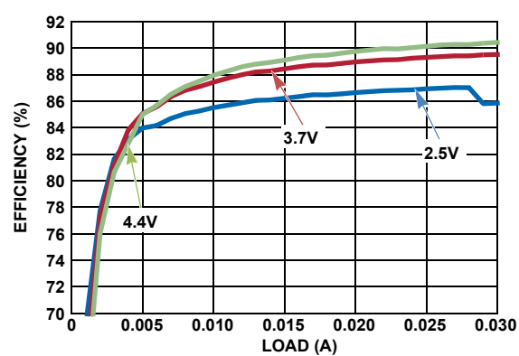
FIGURE 5. DISPLAY POWER SYSTEM EFFICIENCY, V_P/V_N = \pm 5.5\text{V}
