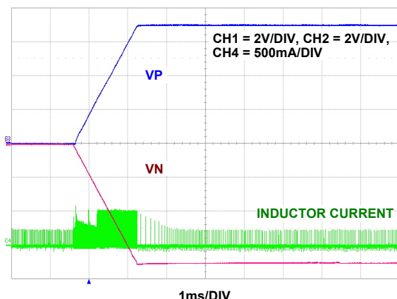
FIGURE 67. VP AND VN ( \pm 7\text{V} ) SOFT-START AT 5V INPUT VOLTAGE, VP/VN START TOGETHER (Reg 0x02 \langle b_6 \rangle = 1 )
