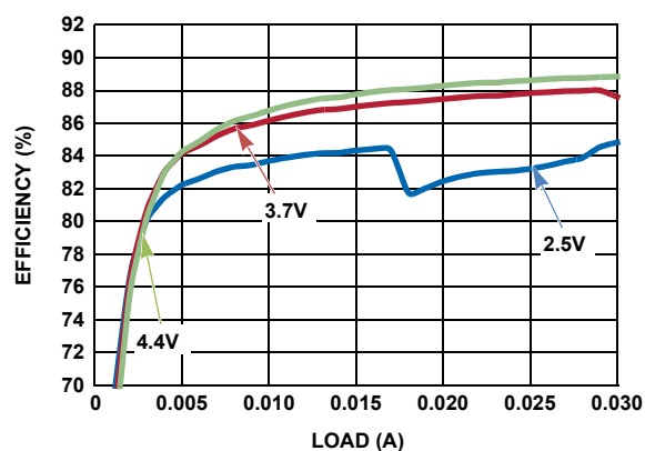
FIGURE 7. DISPLAY POWER SYSTEM EFFICIENCY, V_P/V_N = \pm 7\text{V}
