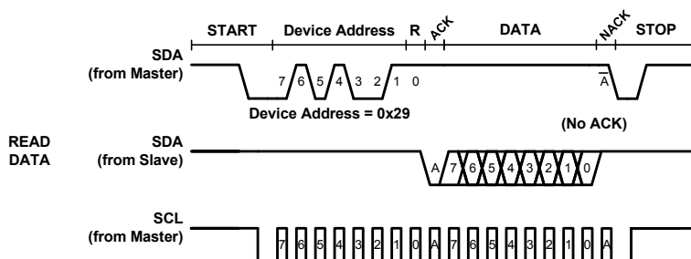
FIGURE 81. I 2 C READ TIMING DIAGRAM
