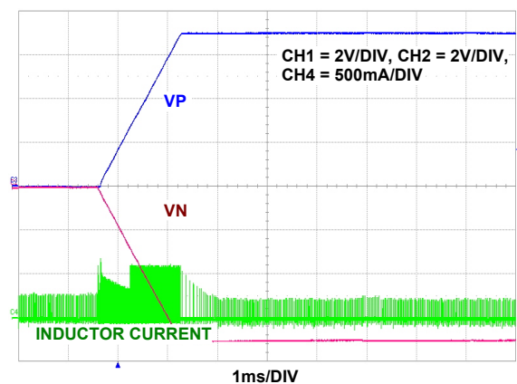
FIGURE 66. VP AND VN ( \pm 7\text{V} ) SOFT-START AT 3.7V INPUT VOLTAGE, VP/VN START TOGETHER (Reg 0x02 \langle b_6 \rangle = 1 )
