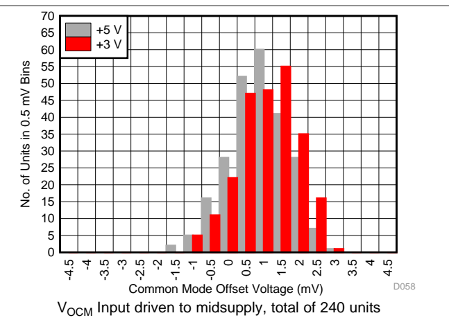
Figure 58. Common-Mode Output Offset from Driven V_{\text{OCM}} Histogram
