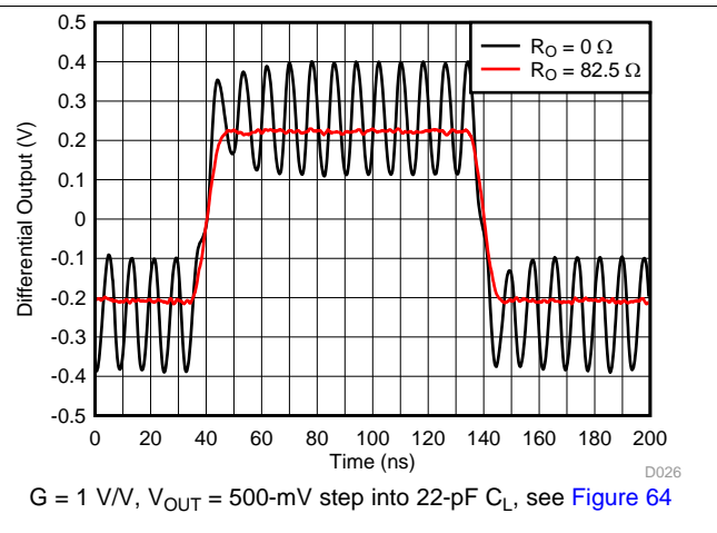
Figure 26. Step Response Into Capacitive Load
