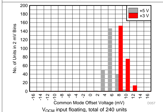
Figure 57. Common-Mode Output Offset from V_{\text{S+}} / 2 Default Value Histogram
