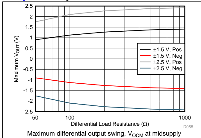
Figure 55. \pm Maximum V_{\text{OUT}} vs Differential Load Resistance
