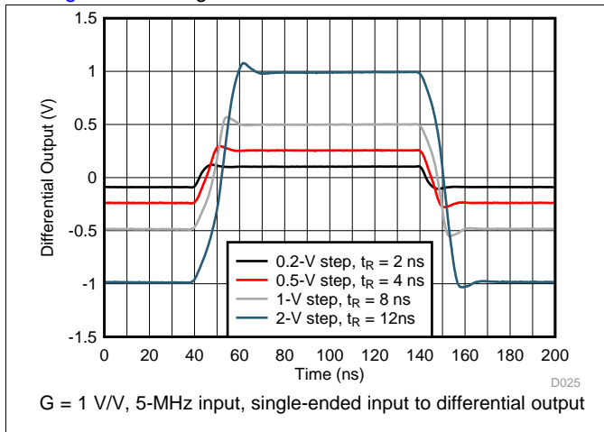
Figure 25. Small- and Large-Signal Step Response
