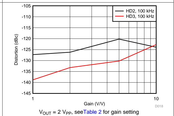
Figure 18. Harmonic Distortion vs Gain
