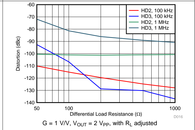
Figure 16. Harmonic Distortion vs R_L
