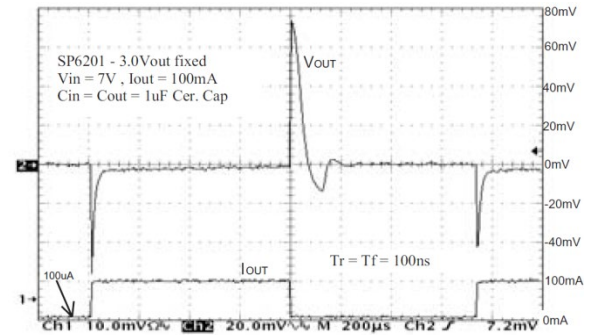
Fig. 33: Load Transient Response, 100mA step, 7\text{V}_{IN}
