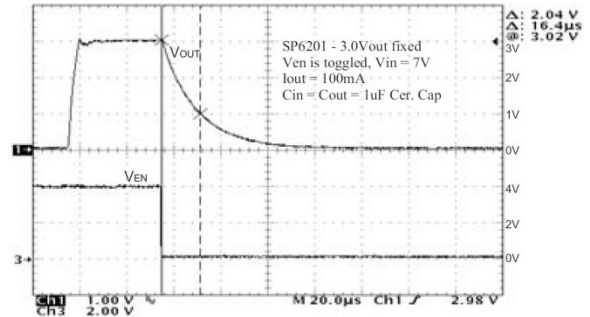
Fig. 29: Turn off time, I_o=100\text{mA} , 7\text{V}_{IN}
