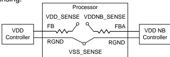
Figure 5. Differential Remote Voltage Sense Connection
