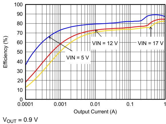
Figure 20. Efficiency With 1.25 MHz
