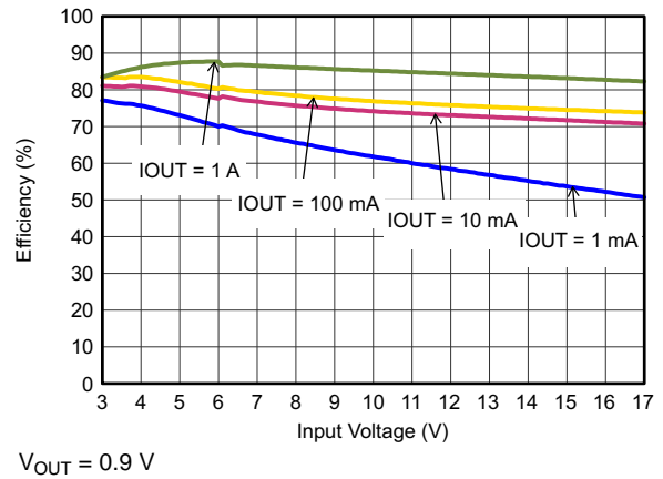
Figure 21. Efficiency With 1.25 MHz
