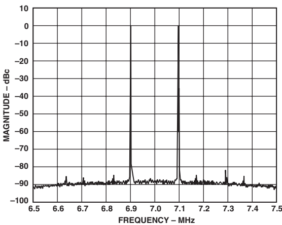
TPC 9. Dual-Tone Spectral Plot @ f_{DATA} = 32 \text{ MSPS} , f_{OUT} = 6.9 \text{ MHz} and 7.1 \text{ MHz} , 4\times \text{LPF}
