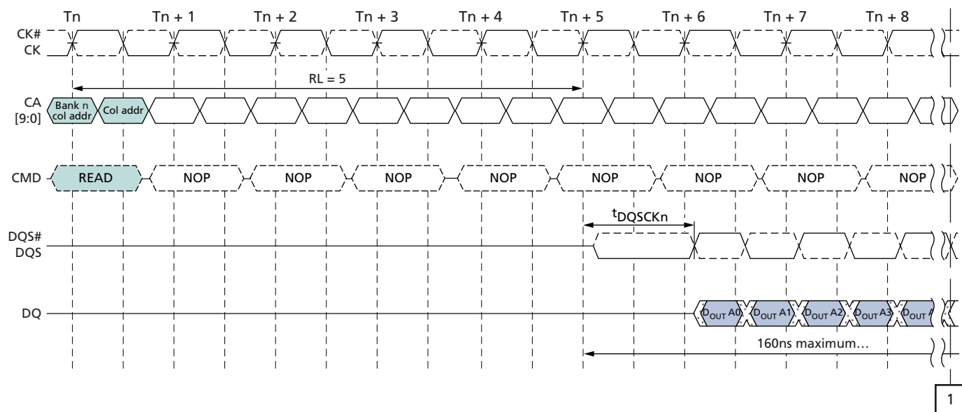
Figure 42: t_{DQSKDS} Timing
