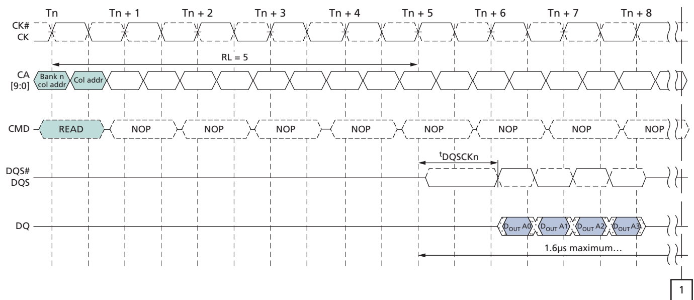
Figure 22: t_{DQSKDM} Timing
