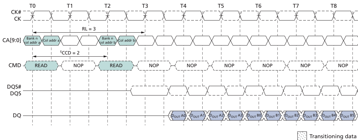
Figure 26: READ Burst Interrupt Example – RL = 3, BL = 8, t_{CCD} = 2
