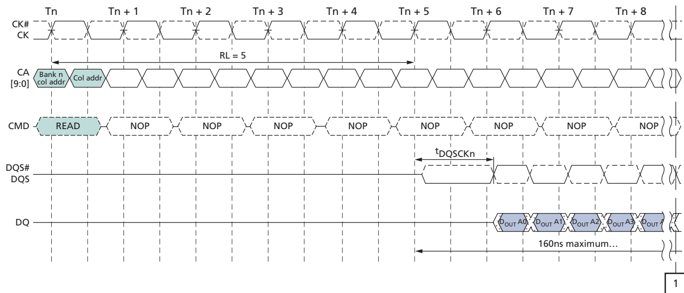
Figure 23: t_{DQSKDS} Timing
