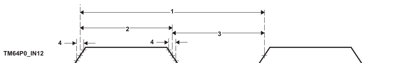
Figure 6-60. Timer Timing
