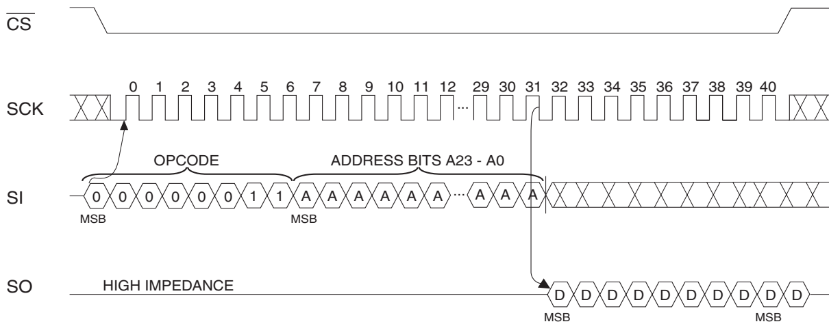
Figure 5-6. READ Timing
