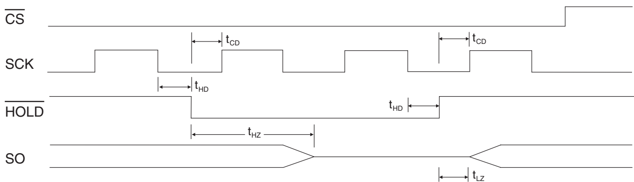
Figure 5-9. HOLD Timing
