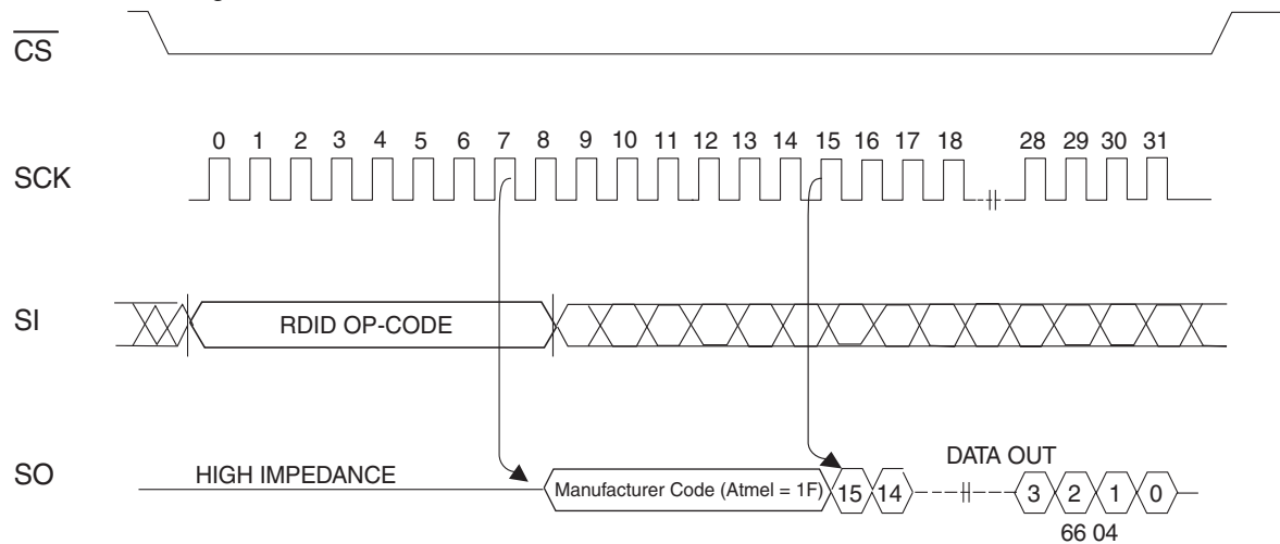
Figure 5-13. RDID Timing
