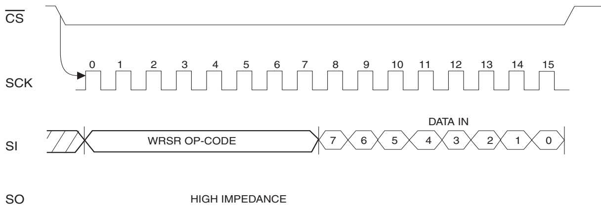
Figure 5-5. WRSR Timing
