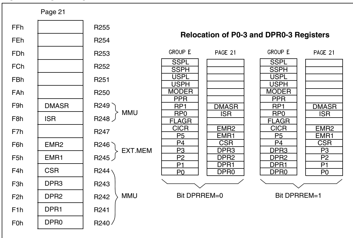
Figure 73. Page 21 Registers
