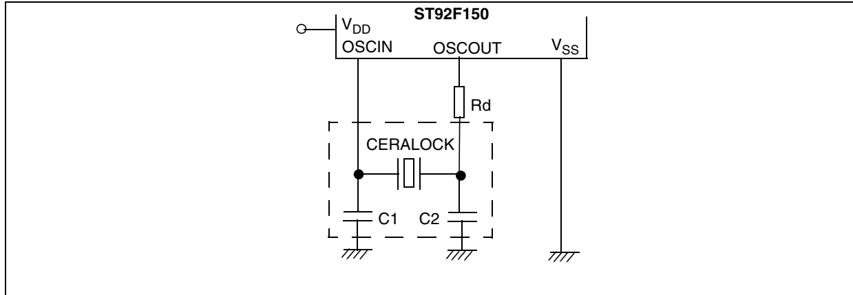
Figure 69. Test Circuit
