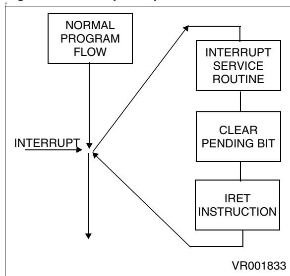
Figure 44. Interrupt Response
