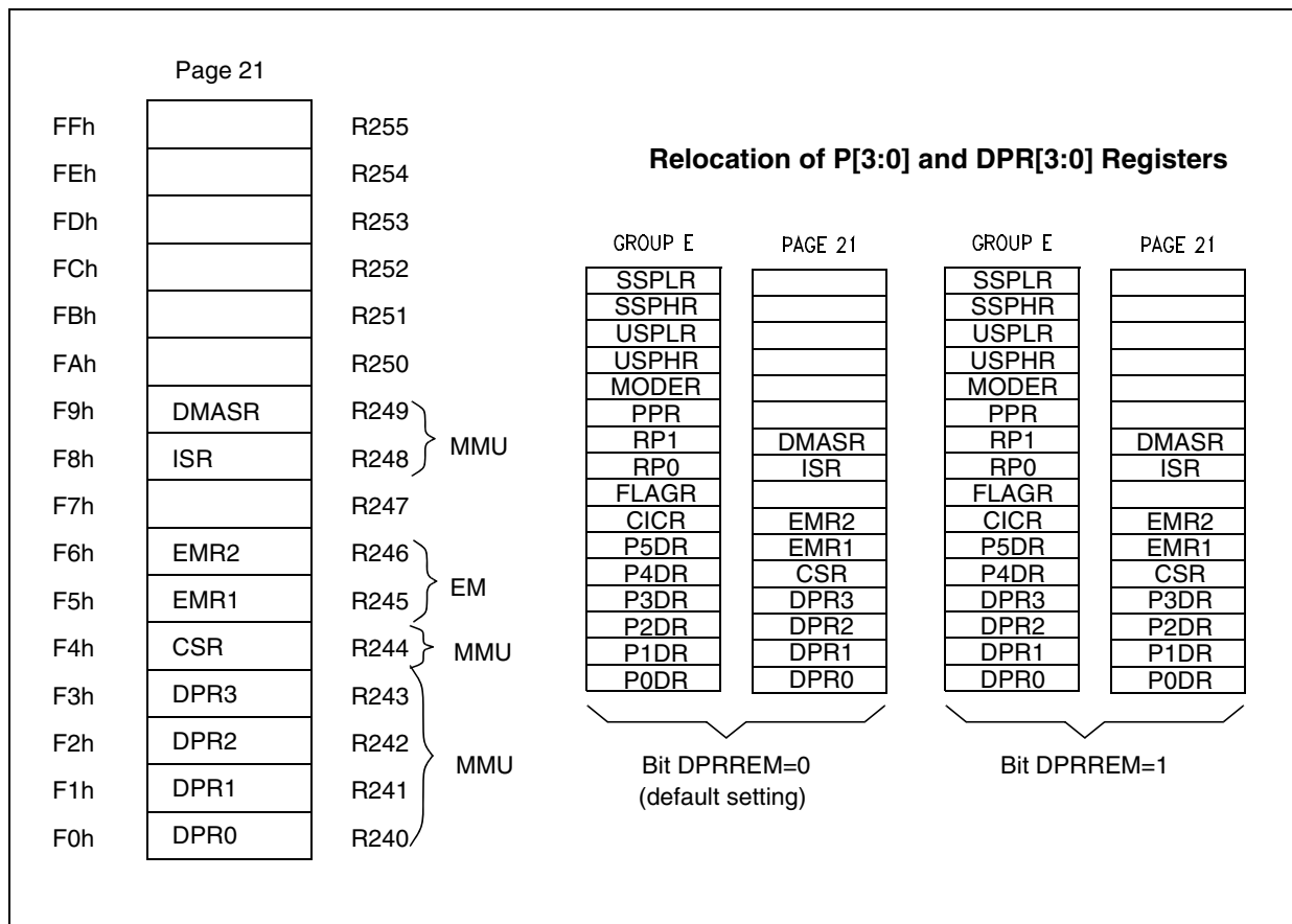
Figure 26. Page 21 Registers
