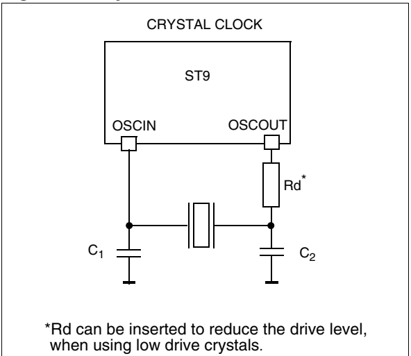
Figure 66. Crystal Oscillator
