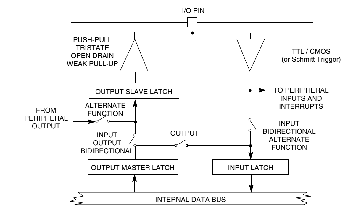
Figure 82. Input Configuration
