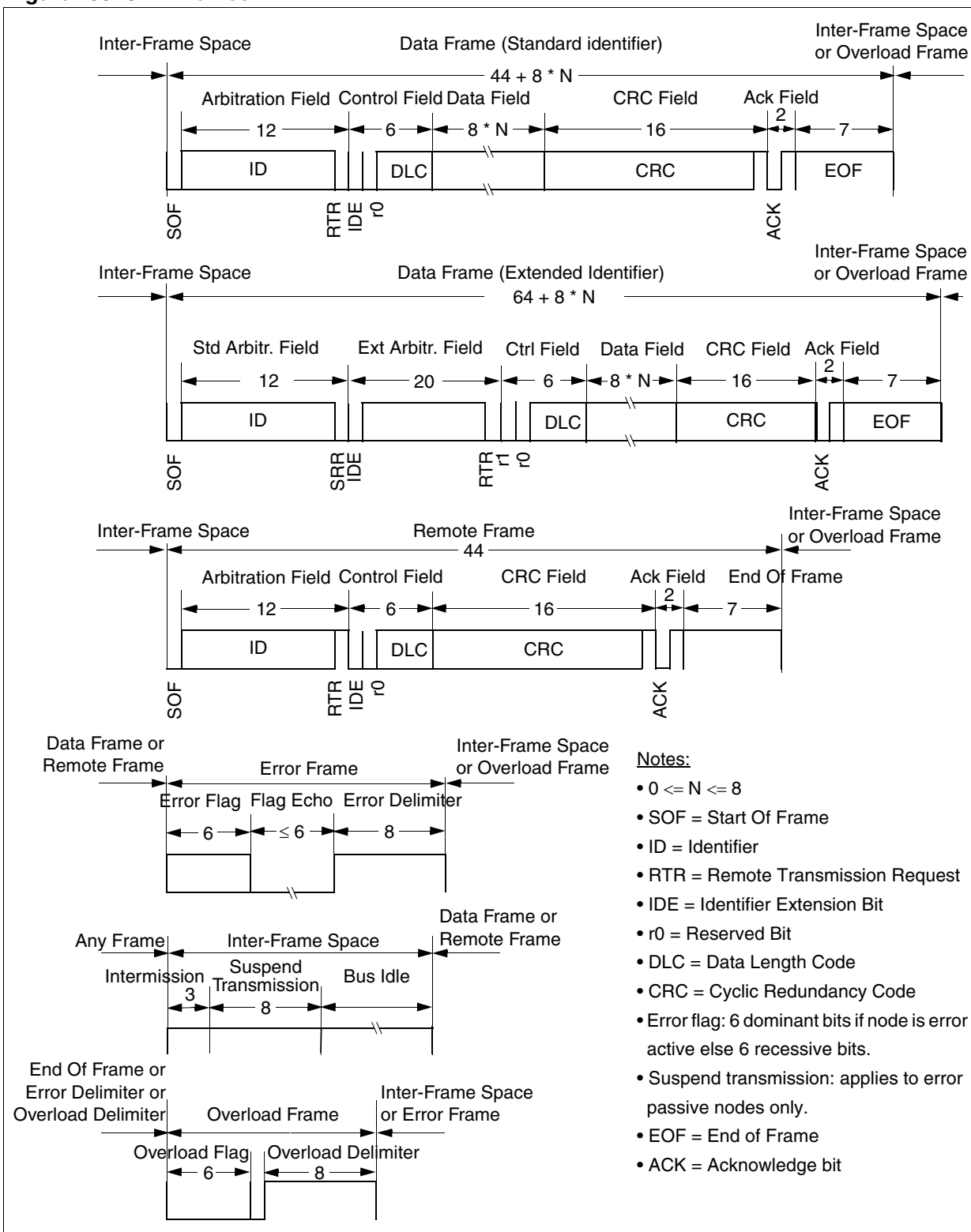
Figure 153. CAN Frames
