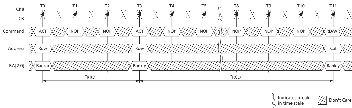
Figure 67: Example: Meeting t_{RRD} (MIN) and t_{RCD} (MIN)
