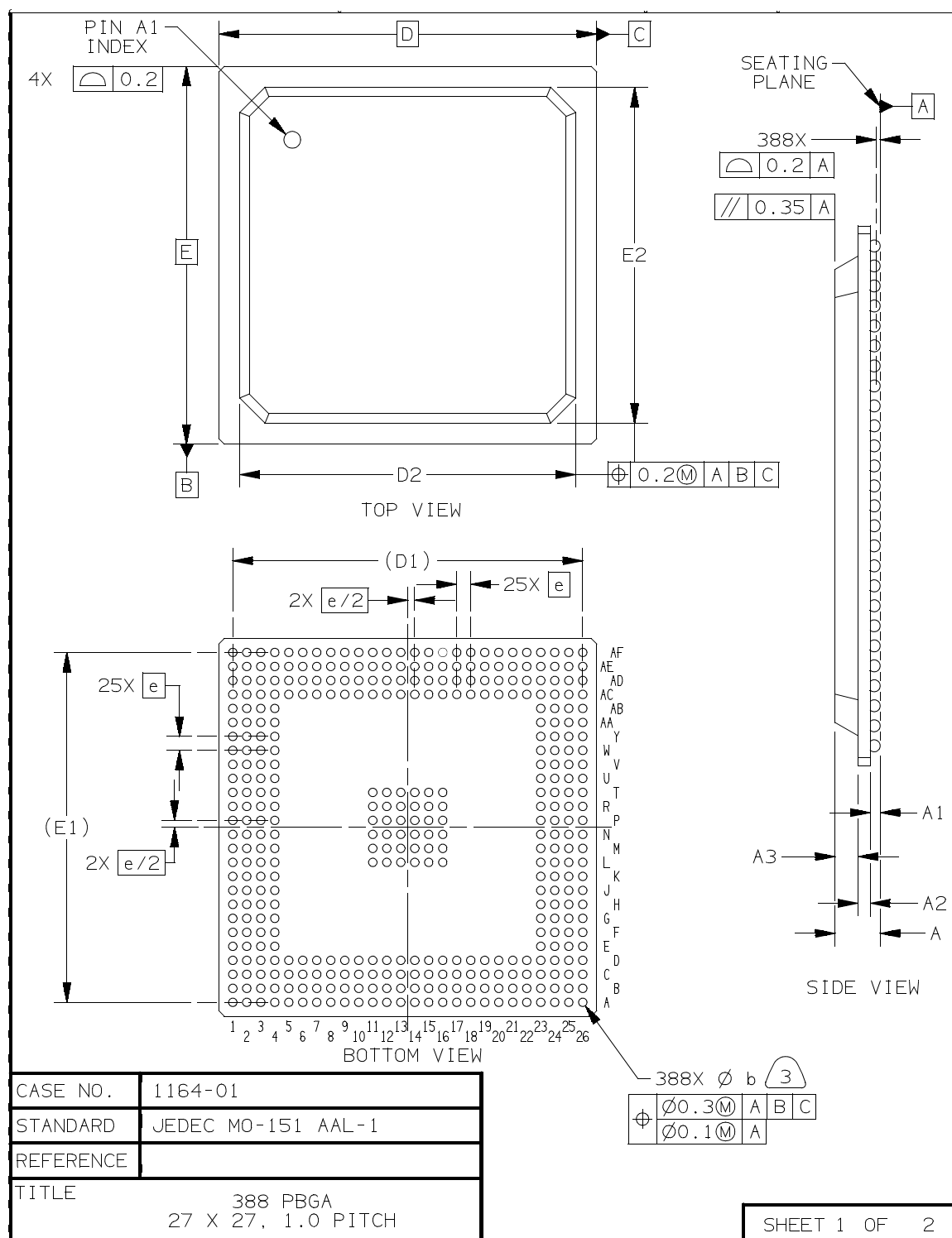
Figure F-64. MPC561/MPC563 Package Footprint (1 of 2)
