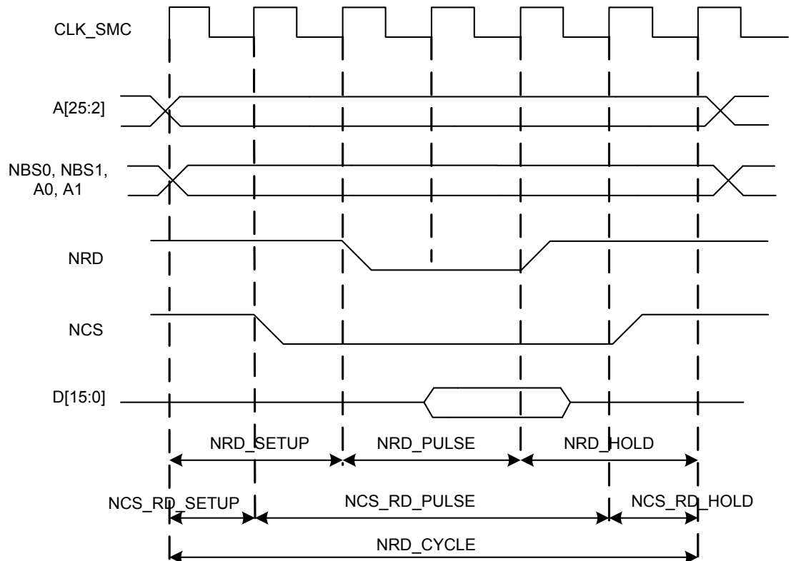
Figure 27-9. Standard Read Cycle
