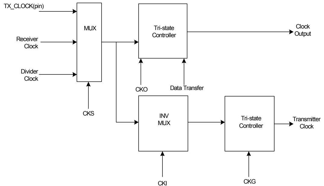
Figure 25-6. Transmitter Clock Management
