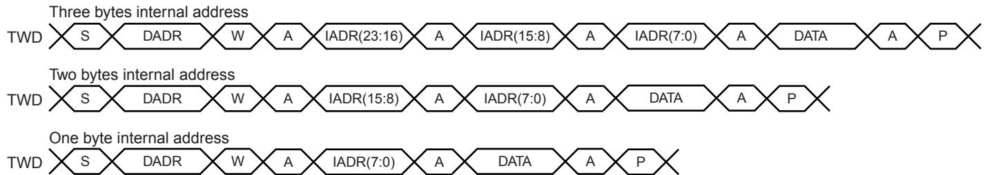
Figure 24-11. Master Write with One, Two or Three Bytes Internal Address and One Data Byte
