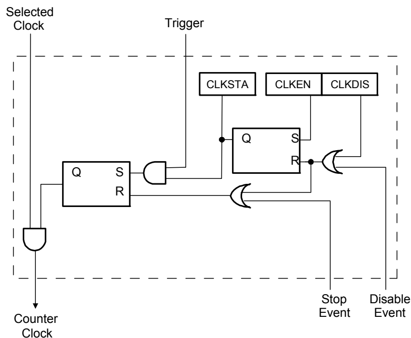
Figure 23-3. Clock Control
