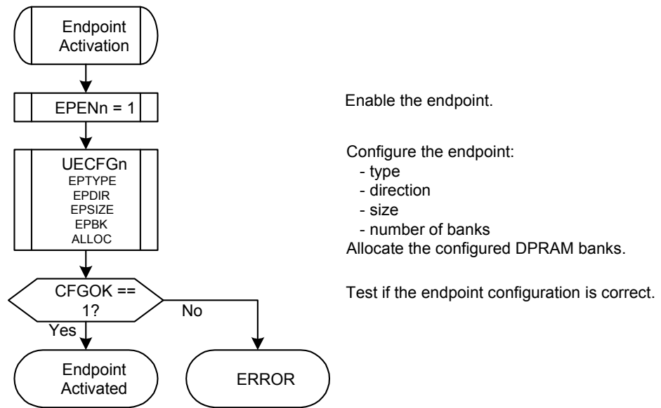
Figure 22-14. Endpoint Activation Algorithm
