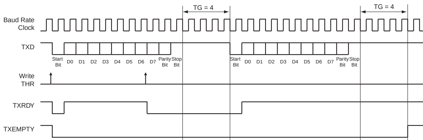
Figure 21-22. Timeguard Operation
