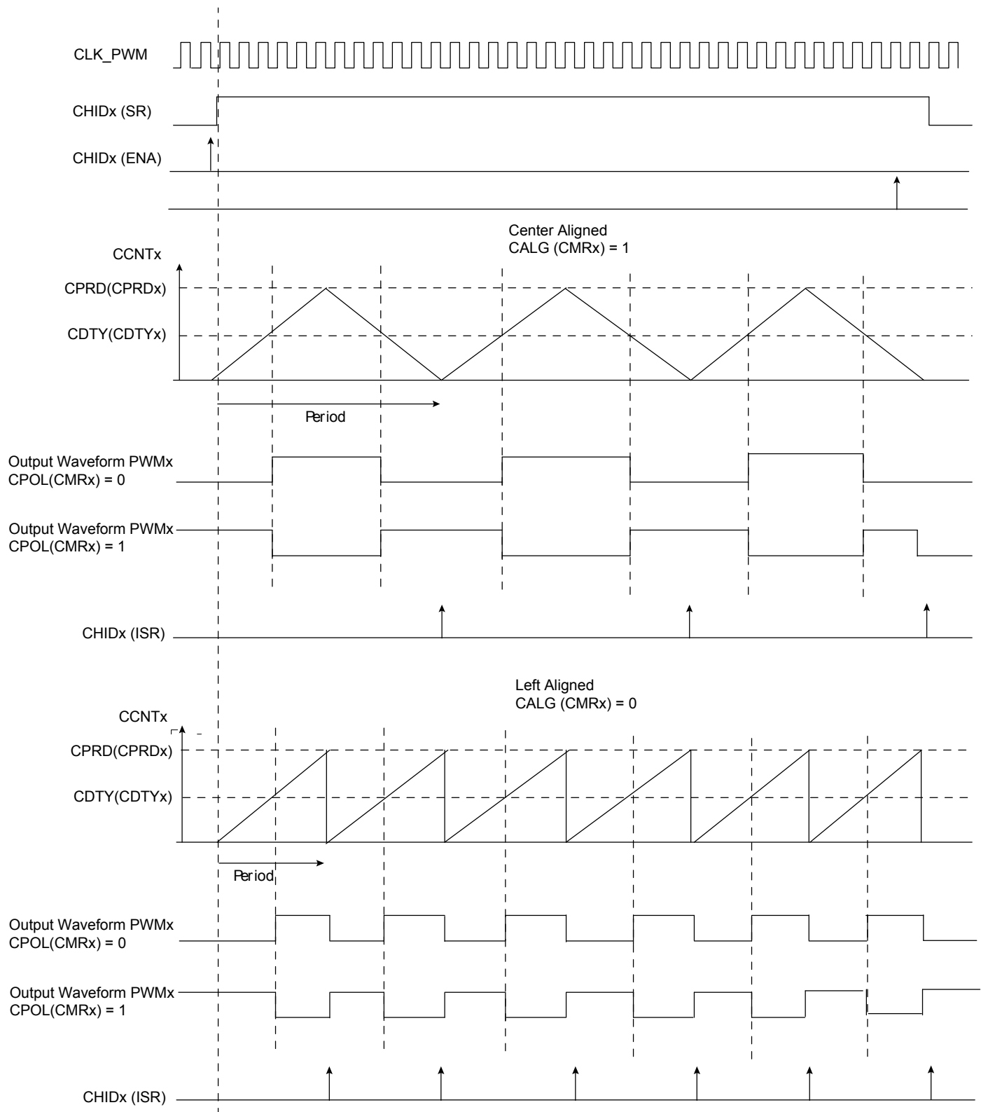
Figure 24-5. Waveform Properties
