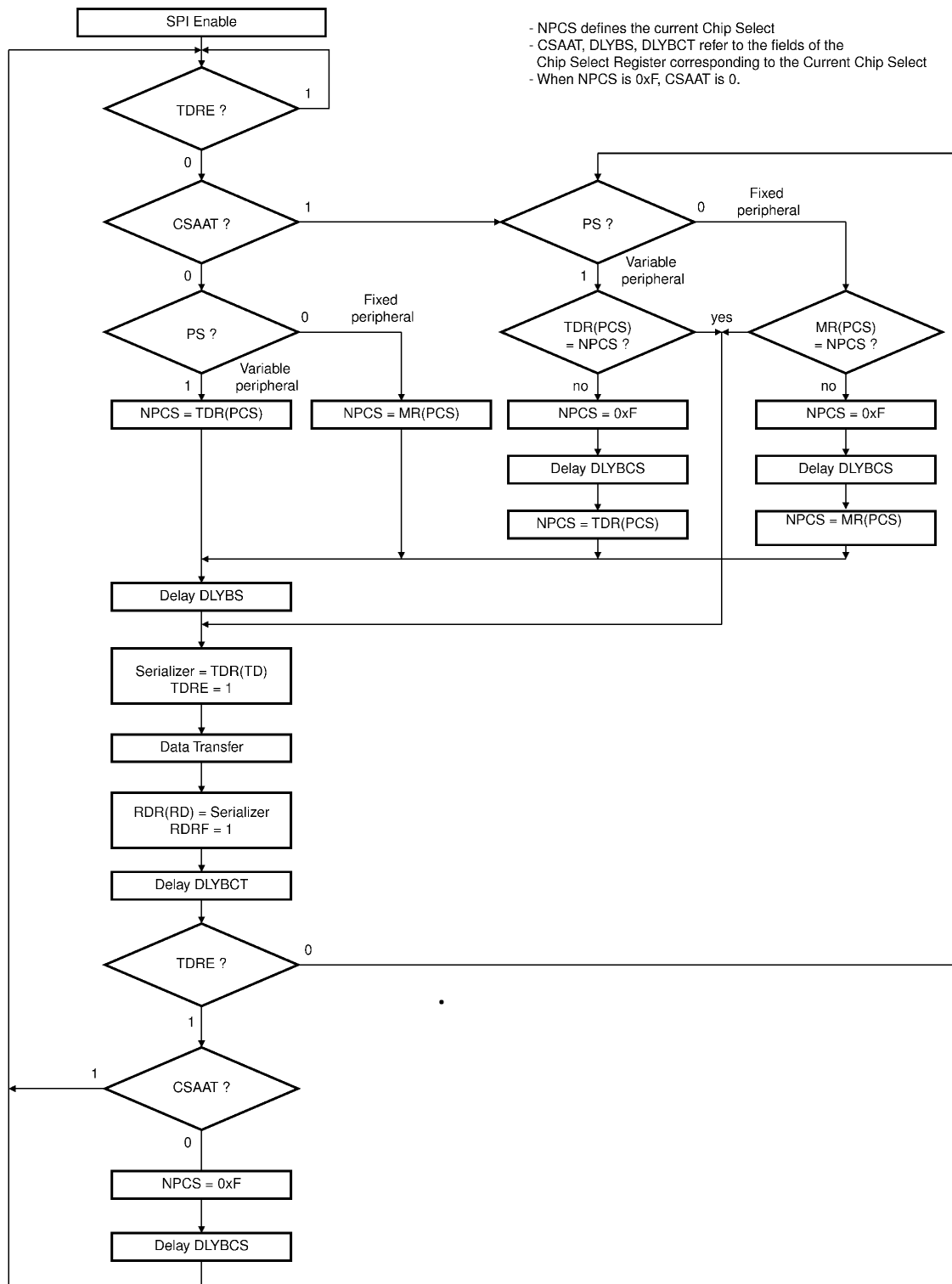
Figure 18-6. Master Mode Flow Diagram
