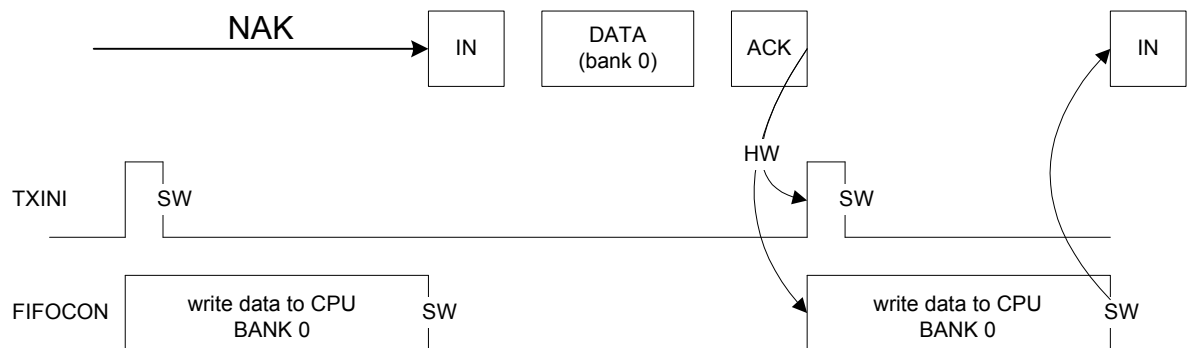
Figure 22-17. Example of an IN Endpoint with 1 Data Bank
