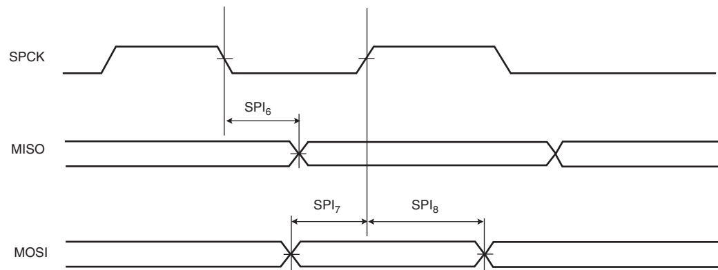
Figure 28-9. SPI Slave mode with (CPOL=0 and NCPHA=1) or (CPOL=1 and NCPHA=0)
