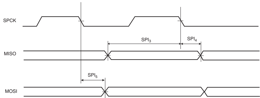
Figure 28-8. SPI Master mode with (CPOL=0 and NCPHA=1) or (CPOL=1 and NCPHA=0)
