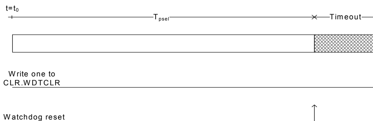
Figure 10-3. Basic Mode WDT Timing Diagram, no clear within T_{psel} .
