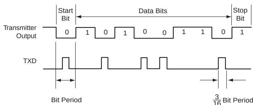
Figure 25-33. IrDA Modulation
