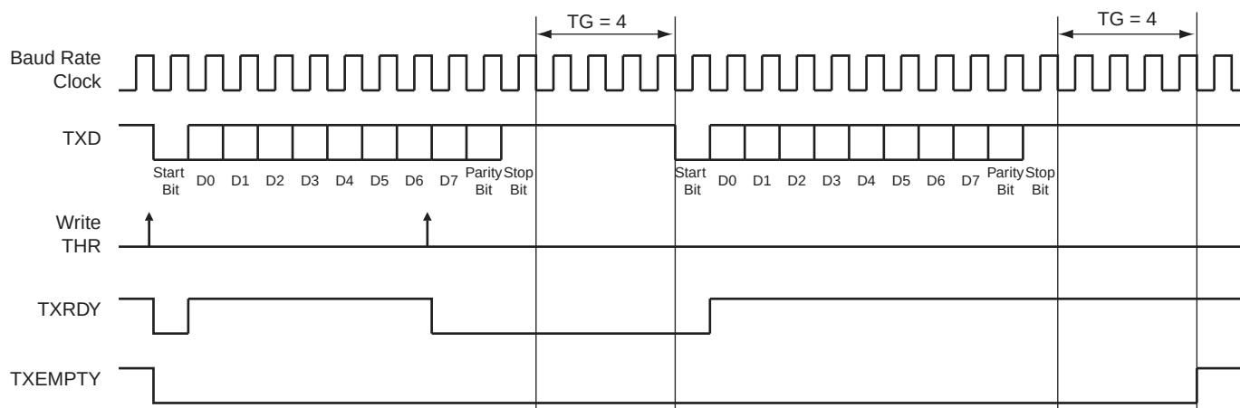
Figure 25-22. Timeguard Operations
