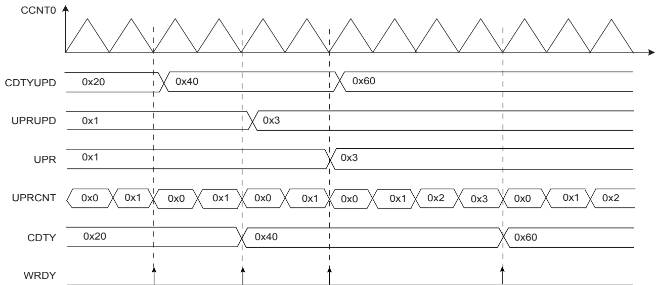
Figure 33-11. Method 2 (UPDM=1)
