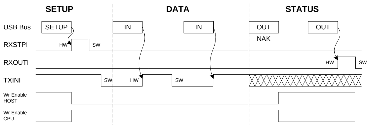
Figure 32-10. Control Read
