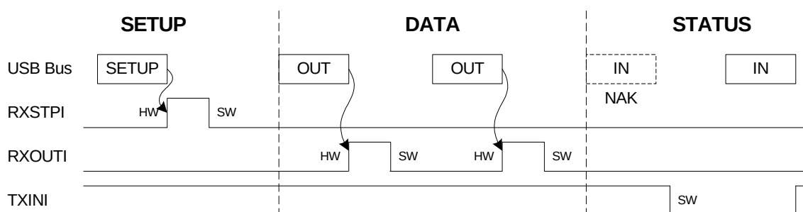
Figure 32-9. Control Write
