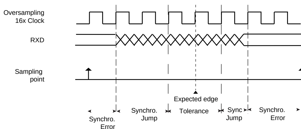
Figure 25-10. Bit Resynchronization
