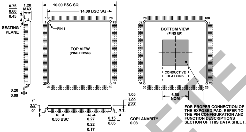
Figure 54. 100-Lead Thin Quad Flat Package, Exposed Pad [TQFP_EP] (SV-100) Dimensions shown in millimeters
