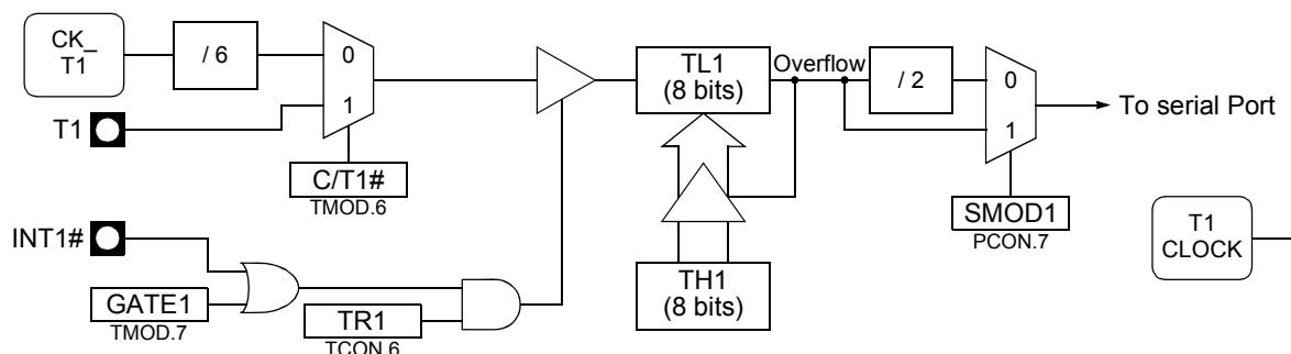
Figure 67. Timer 1 Baud Rate Generator Block Diagram
