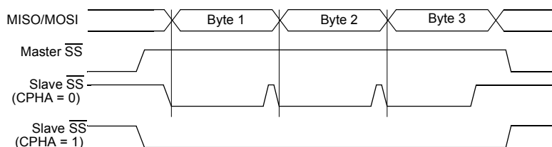
Figure 87. CPHA/ \overline{SS} Timing
