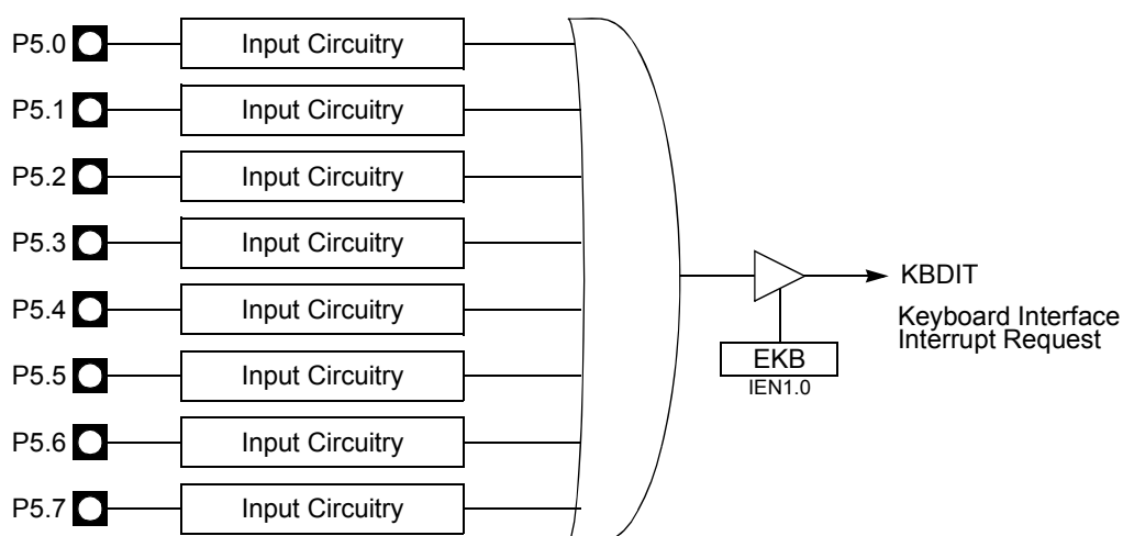
Figure 98. Keyboard Input Circuitry
