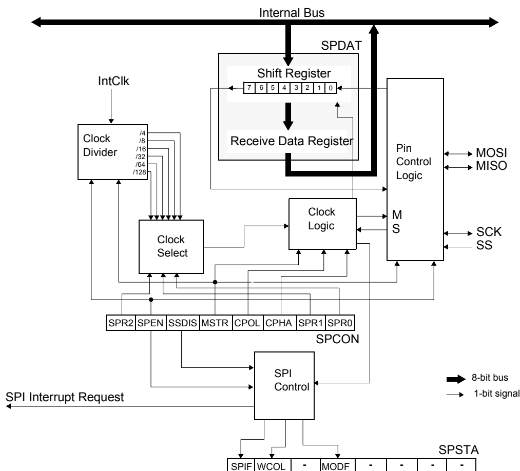
Figure 83. SPI Module Block Diagram
