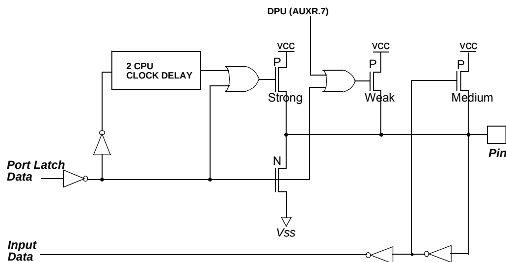
Figure 23. Quasi Bi-directional Port
