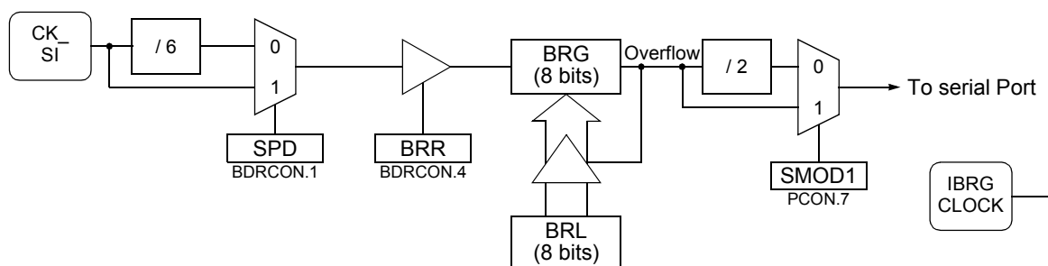
Figure 68. Internal Baud Rate Generator Block Diagram
