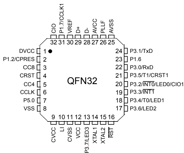
Figure 7. QFN32 Package Pinout
