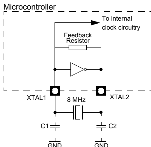
Figure 15. Oscillator Schematic
