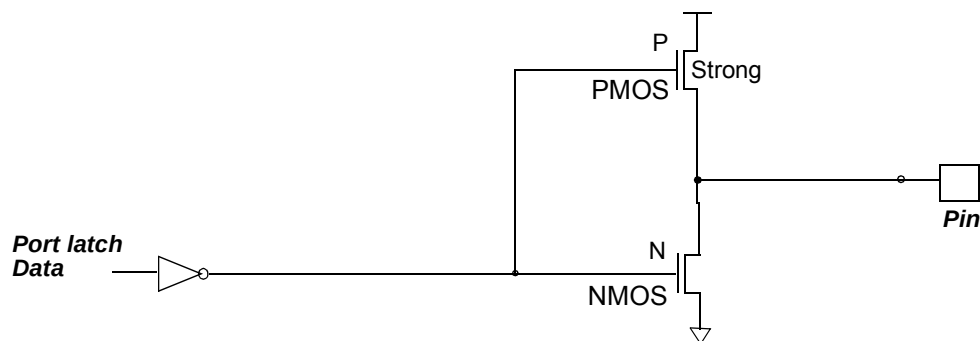
Figure 24. Push-pull Output
