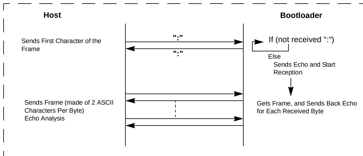
Figure 47. Command Flow
