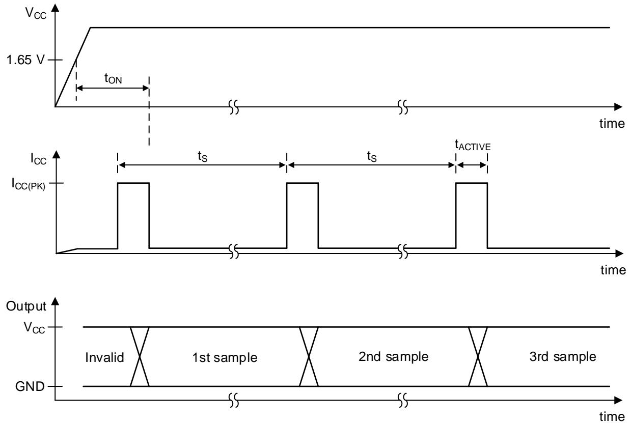
Figure 17. Timing Diagram
