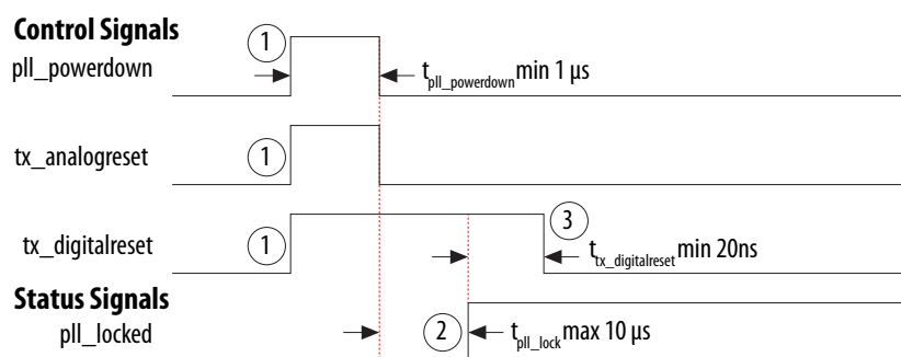
Figure 3-6: Reset Sequence Timing Diagram for Transmitter using the User-Coded Reset Controller during Device Operation
