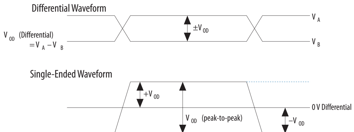
Figure 1-17: VOD (Differential) Signal Level
