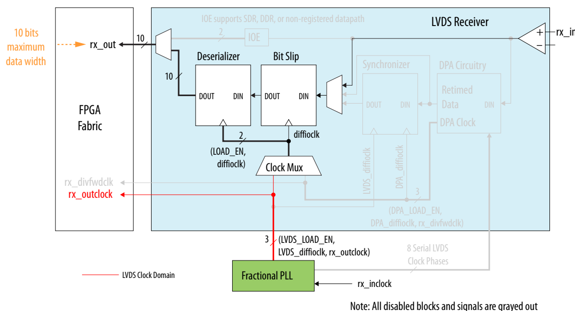
Figure 6-24: Receiver Data Path in Non-DPA Mode
