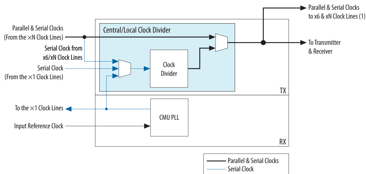
Figure 2-12: Clock Dividers
