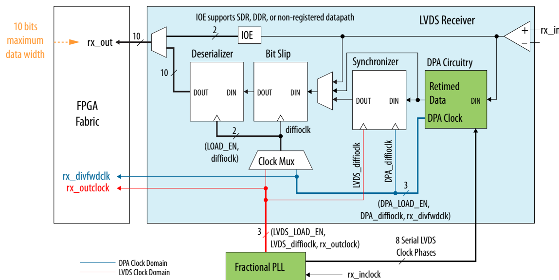
Figure 6-19: Receiver Block Diagram
