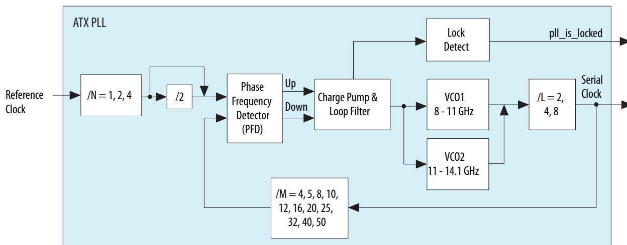
Figure 1-16: ATX PLL Architecture
