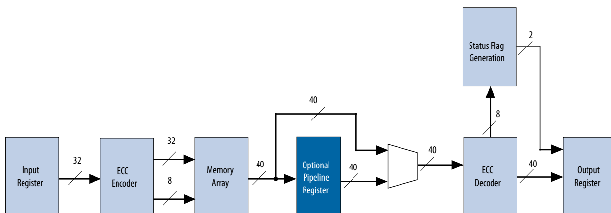
Figure 2-11: ECC Block Diagram for M20K Memory
