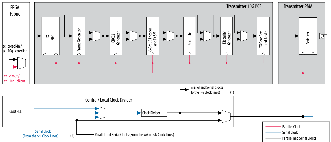
Figure 2-14: Transmitter 10G PCS and PMA Clocking
