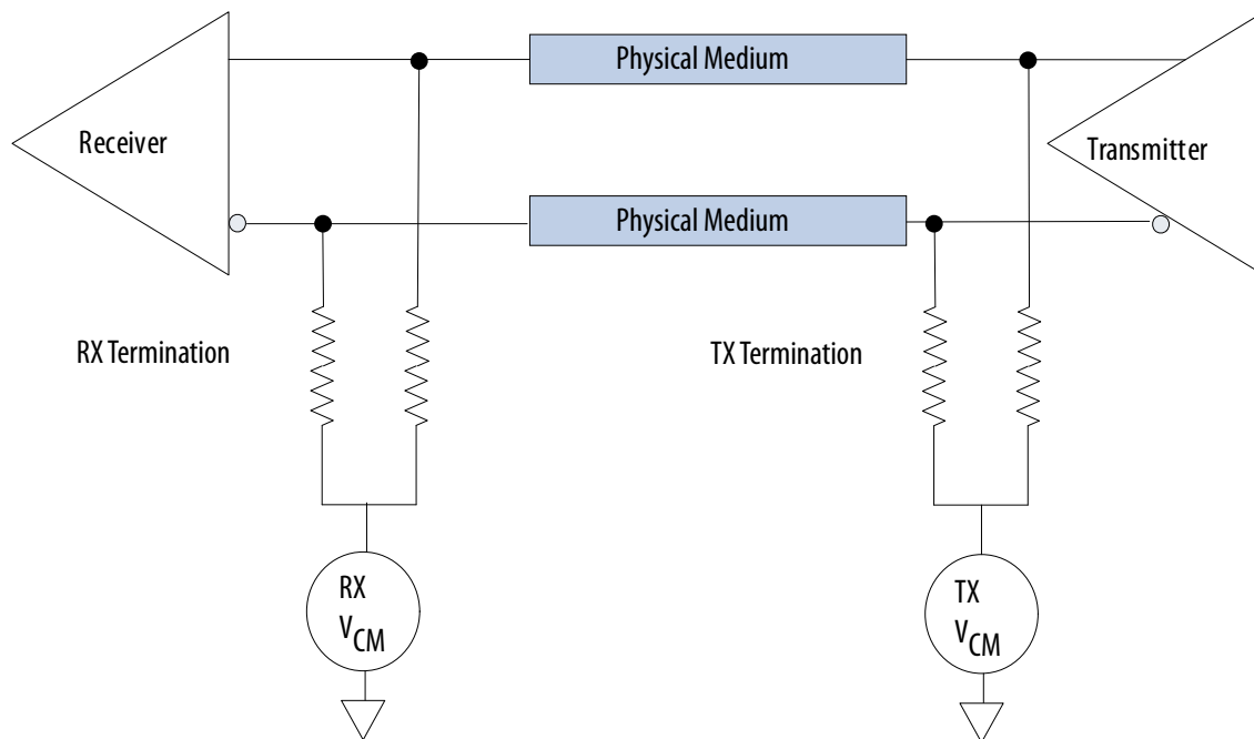
Figure 1-18: DC-Coupled Link
