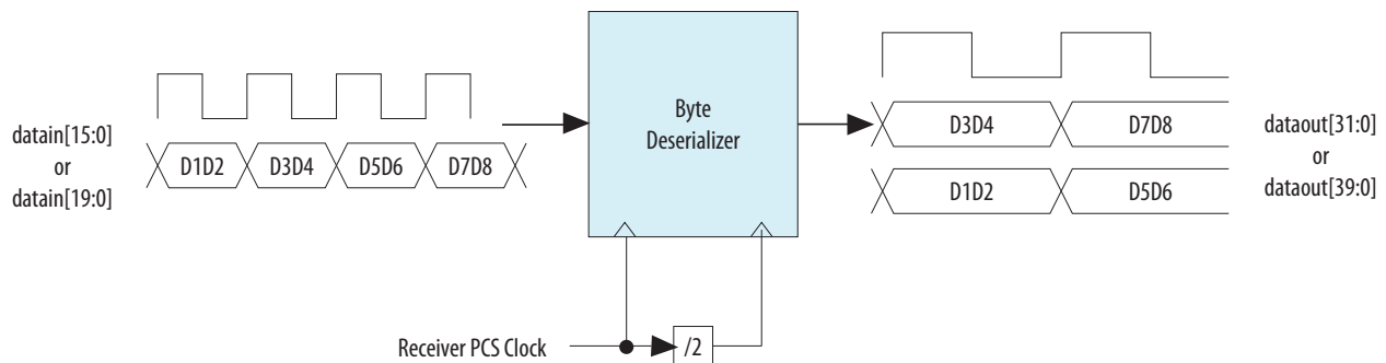
Figure 1-25: Byte Deserializer in 16- and 20-Bit Width Mode
