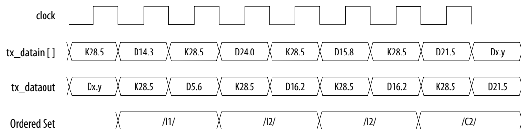
Figure 4-9: Example of Automatic Ordered Set Generation
