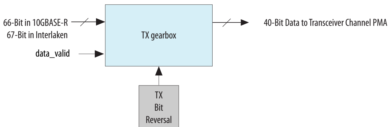
Figure 1-39: Transmitter Gearbox
