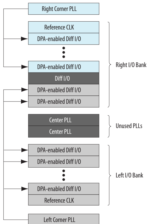
Figure 6-11: Corner PLLs Driving DPA-enabled Differential I/Os
