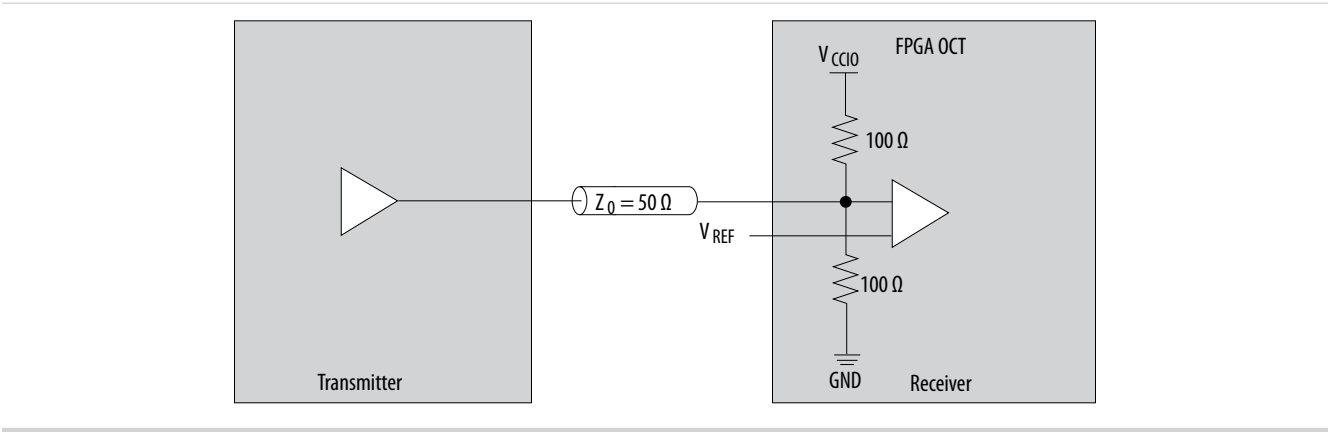
Figure 5-7: R_T OCT with Calibration
