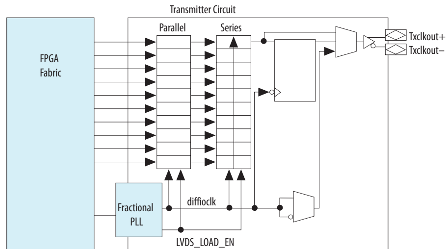
Figure 6-15: Transmitter in Clock Output Mode
