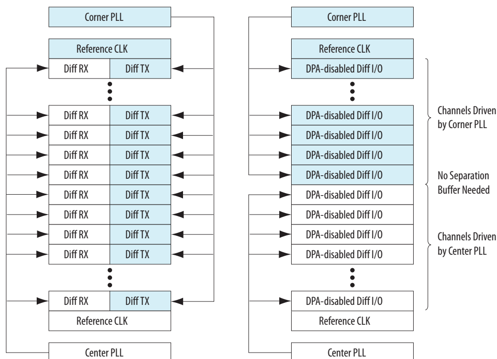
Figure 6-12: Corner and Center PLLs Driving DPA-Disabled Differential I/Os in the Same Bank
