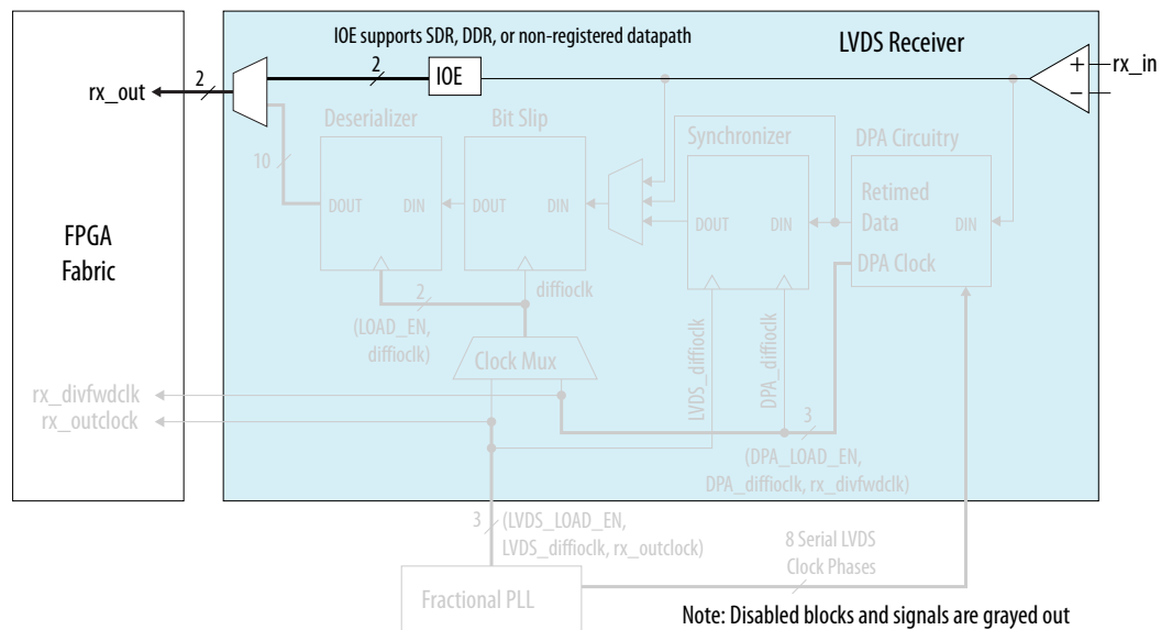
Figure 6-23: Deserializer Bypass
