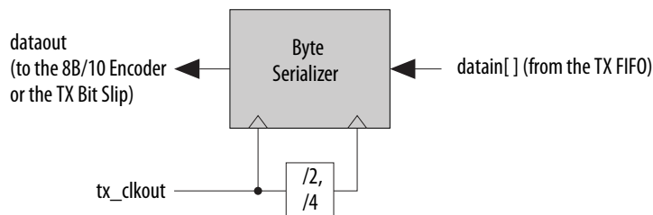
Figure 1-29: Transmitter Phase Compensation FIFO
