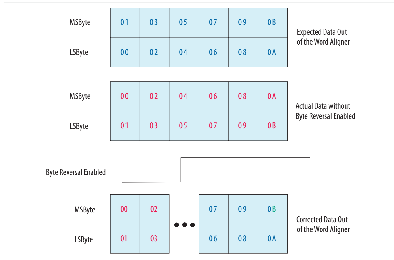
Figure 1-22: Receiver Byte Reversal Feature
