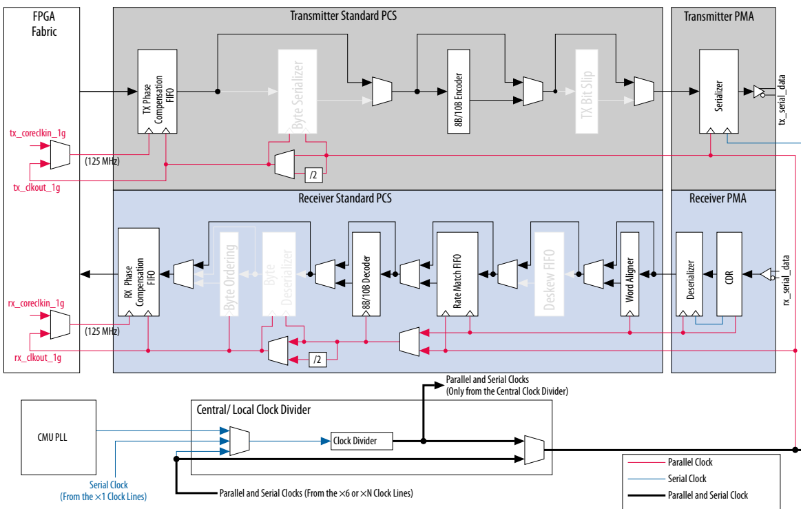
Figure 4-8: 1000BASE-X and 1000BASE-KX Datapath Configurations
