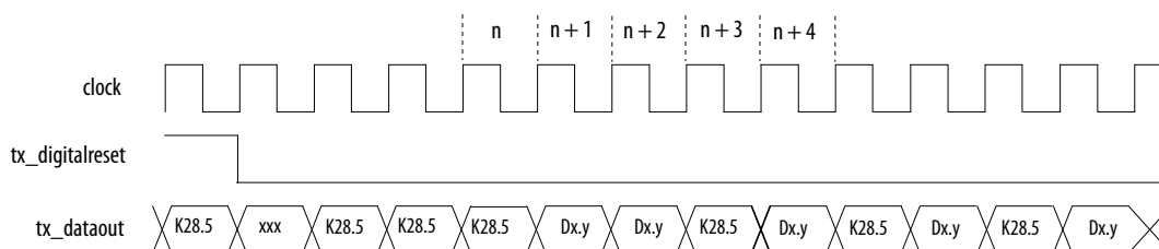
Figure 4-10: Example of Reset Condition in 1000BASE-X and 1000BASE-KX Configurations
