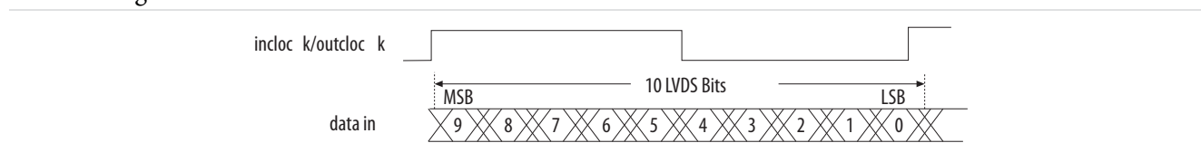
Figure 6-28: Bit Orientation in the Quartus II Software
