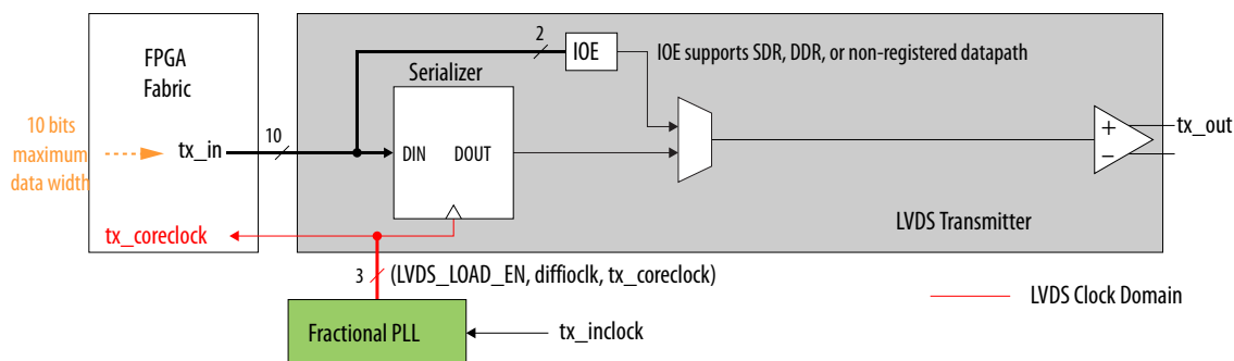
Figure 6-14: LVDS Transmitter
