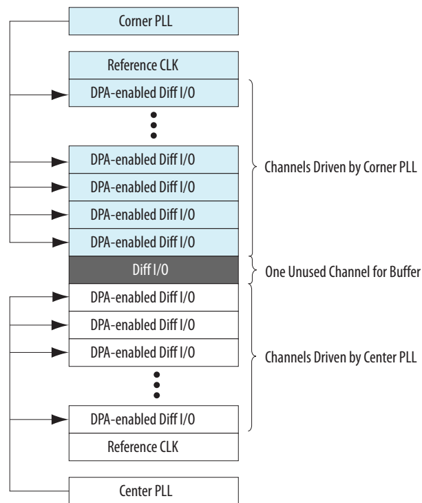
Figure 6-8: Center and Corner PLLs Driving DPA-enabled Differential I/Os in the Same Bank
