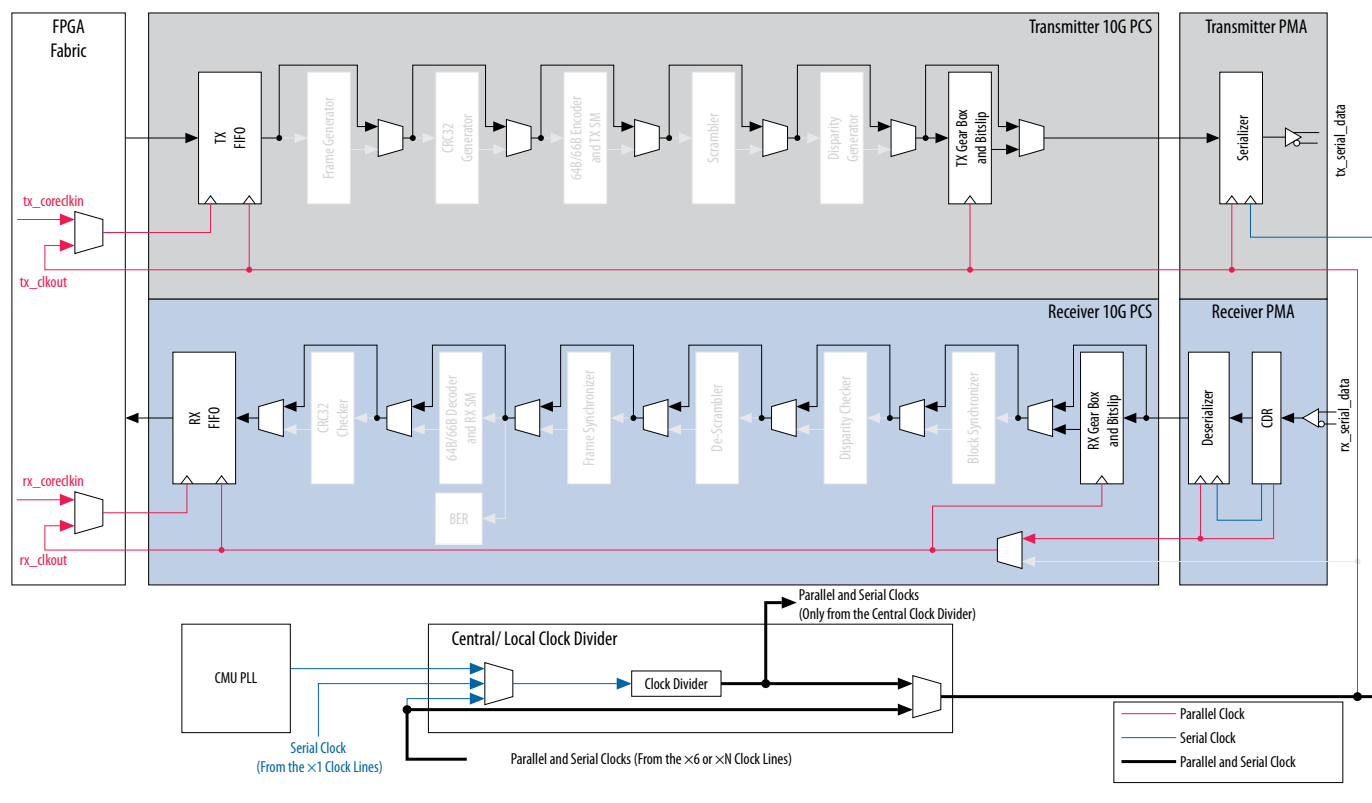
Figure 4-65: 10G PCS Low Latency Configuration Datapath
