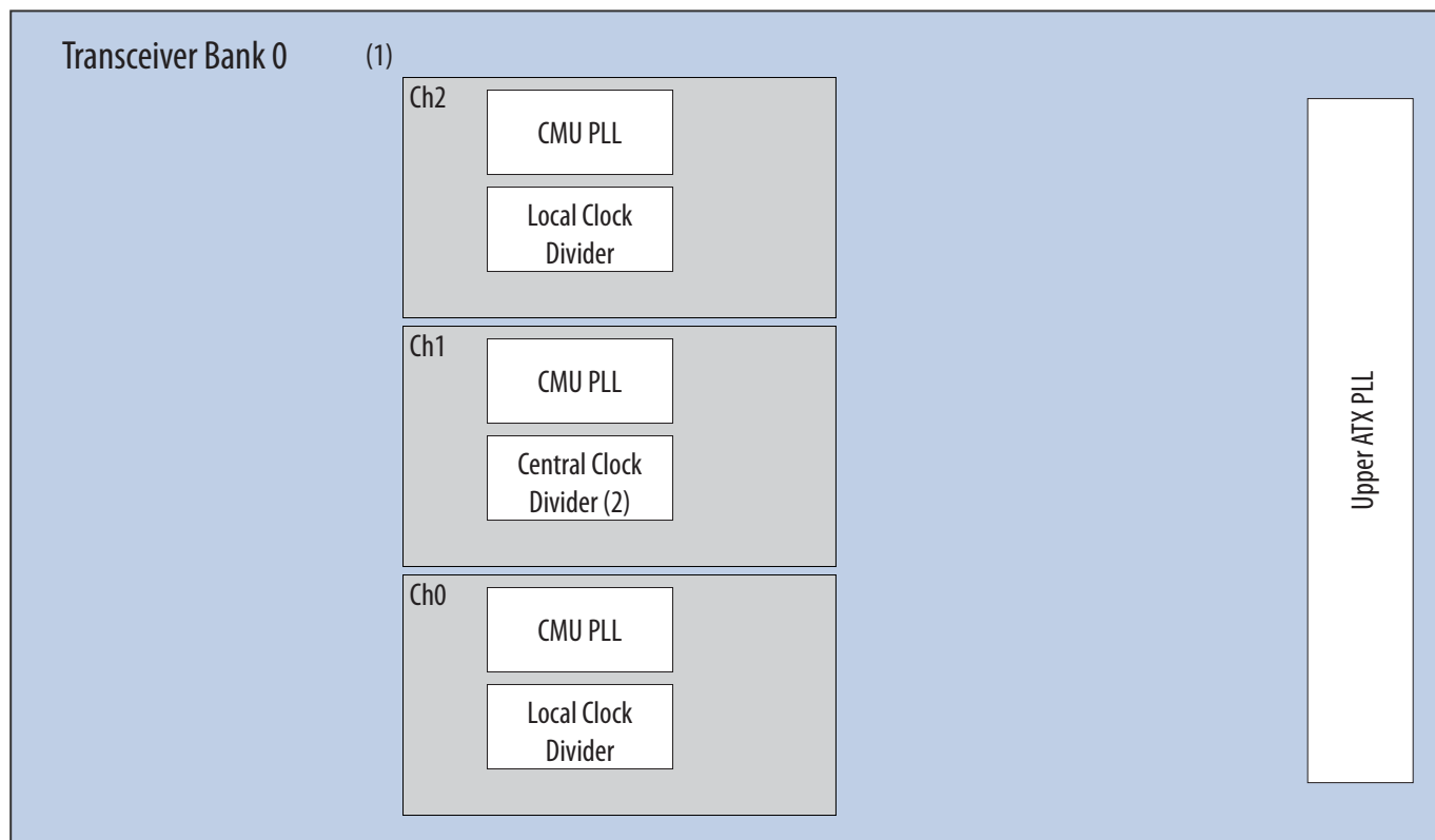
Figure 1-12: Transmitter PLL Locations in GX Devices (3 Channels)
