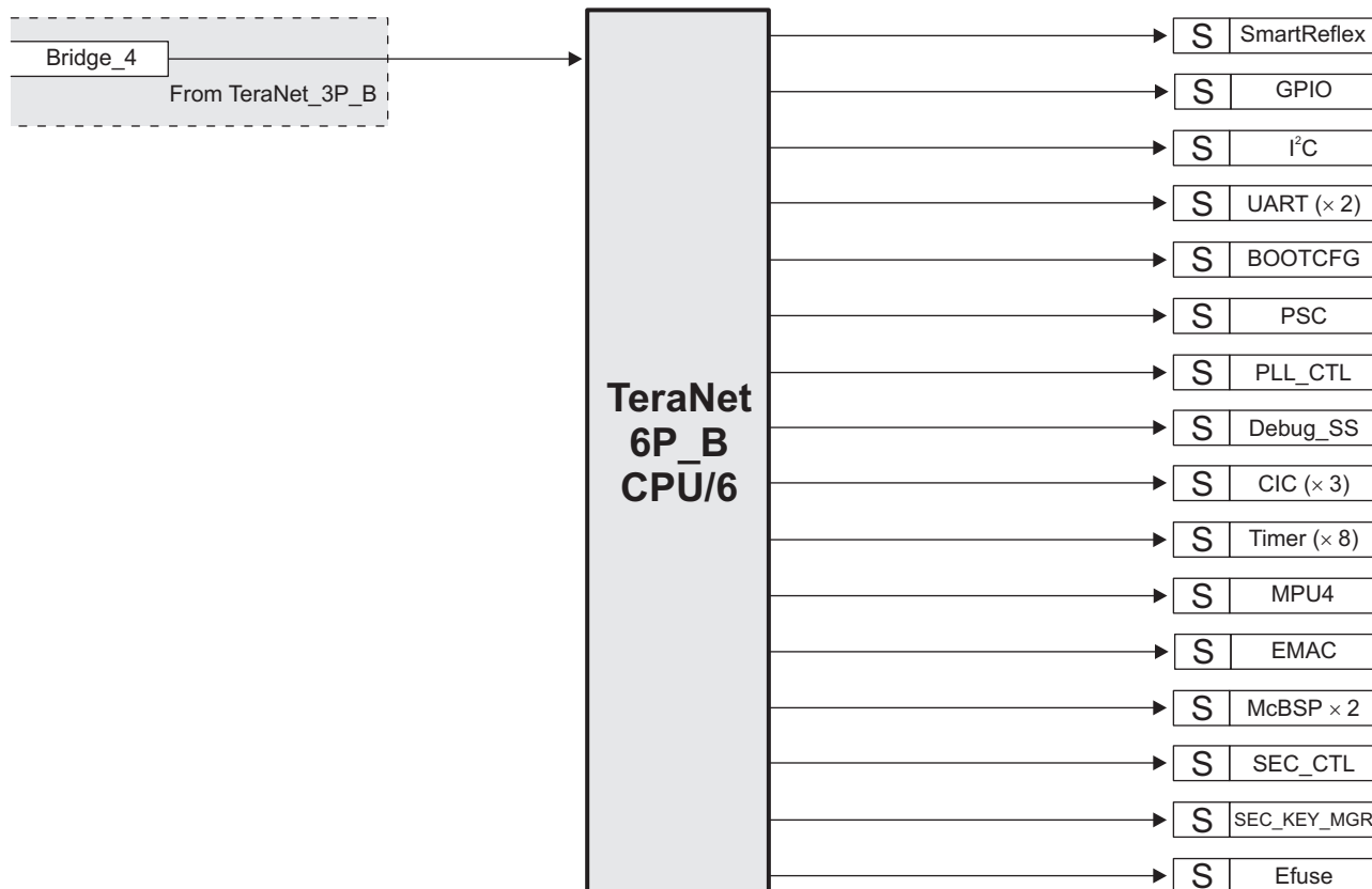
Figure 9-5. TeraNet 6P_B
