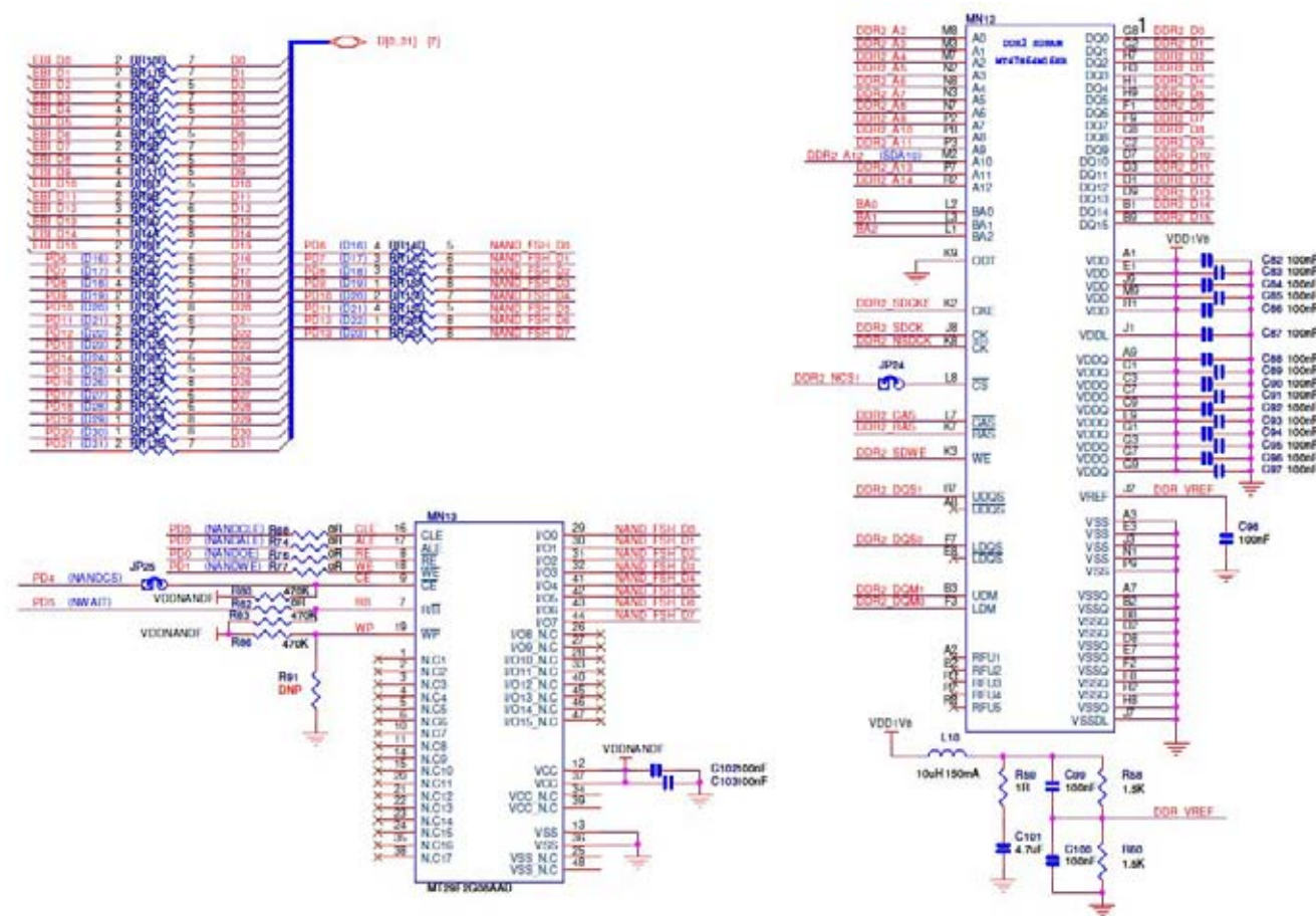
Figure 25-13. Hardware Configuration - 8-bit NAND Flash with NFD0 ON D16 = 1
