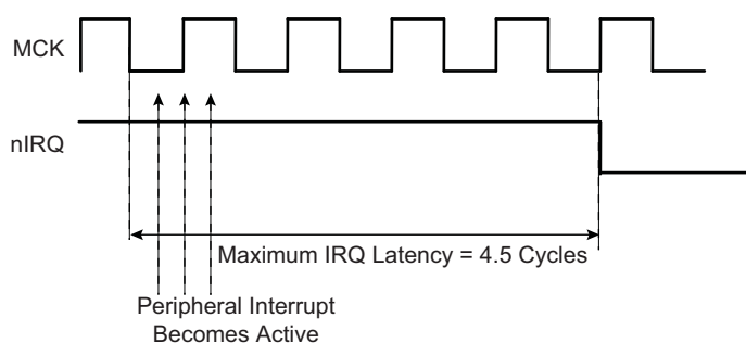
Figure 12-8. Internal Interrupt Edge Triggered Source
