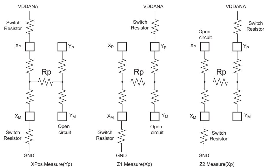
Figure 40-8. Pressure Measurement
