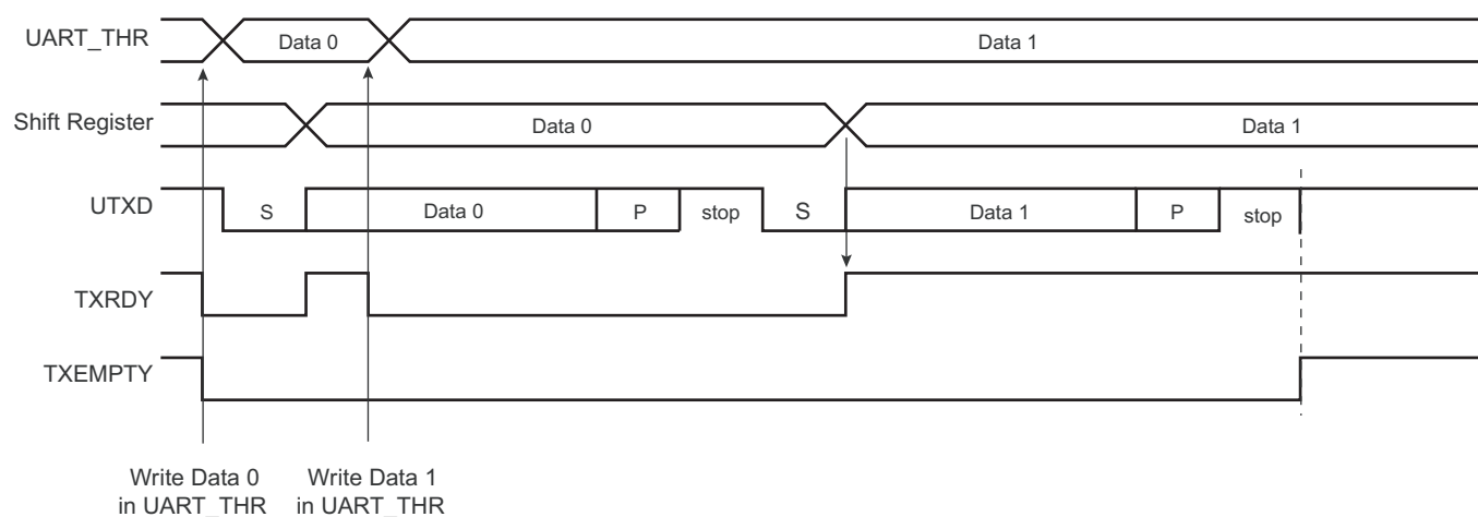
Figure 39-10. Transmitter Control
