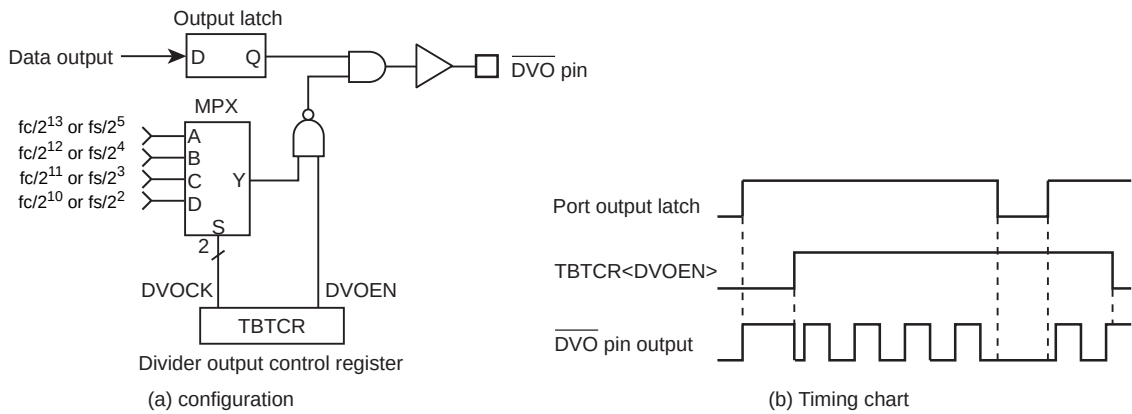
Figure 9-3 Divider Output
