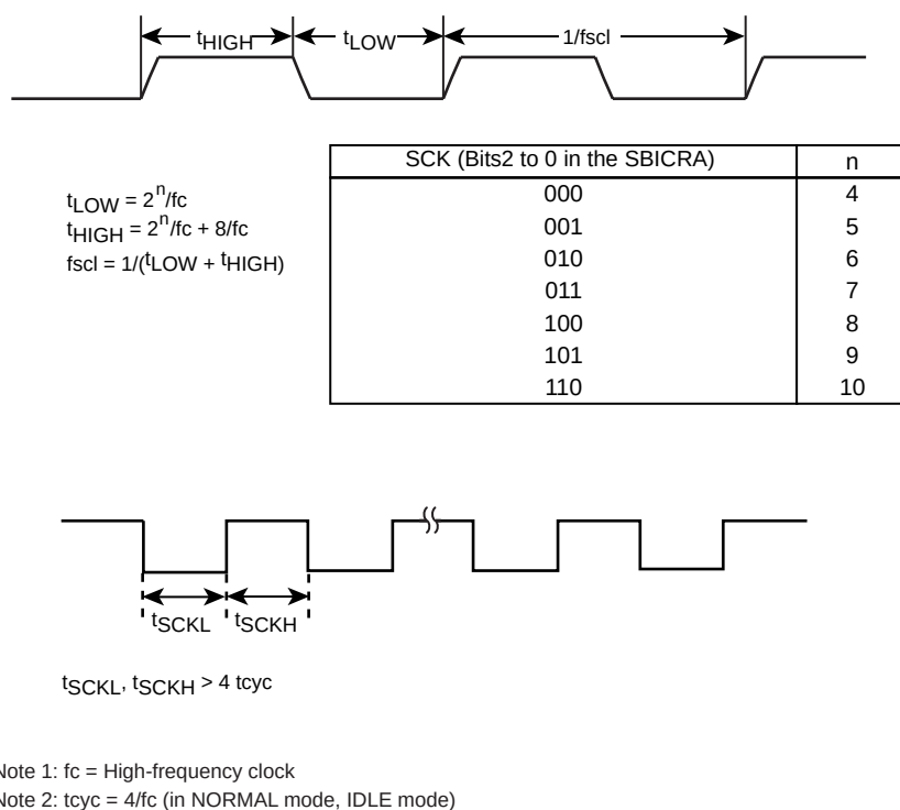
Figure 15-3 Clock Source
