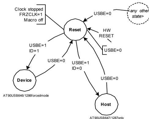
Figure 22-9. USB controller states after reset.
