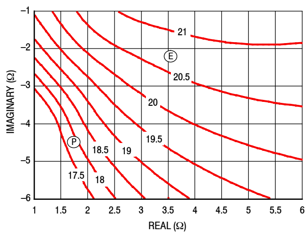
Figure 10. P1dB Load Pull Gain Contours (dB)
