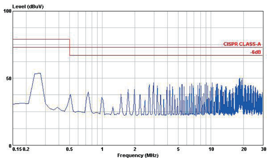
Conducted Emission EN55032 Class A
