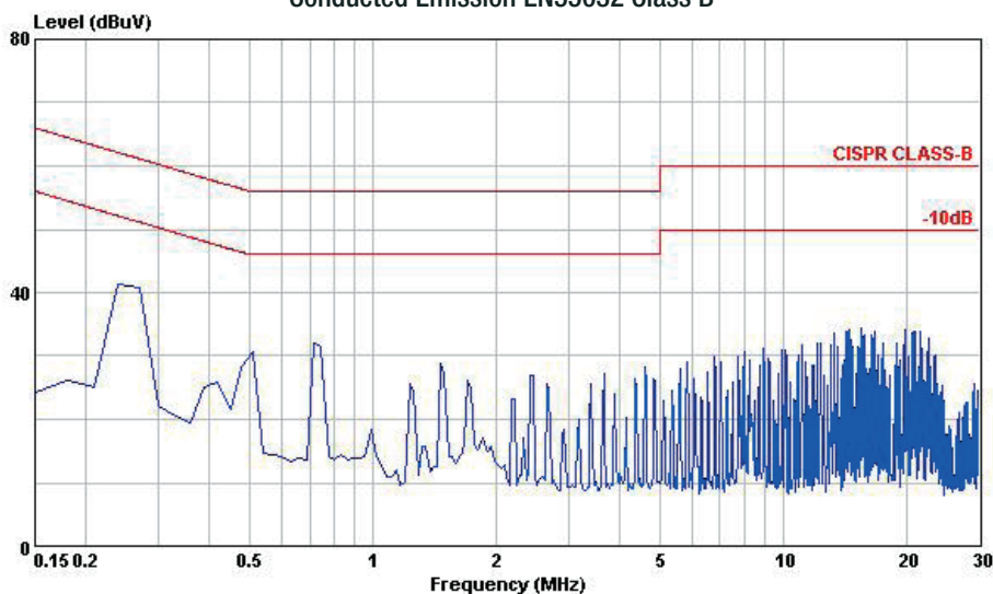
Conducted Emission EN55032 Class B
