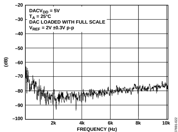
Figure 22. DAC Total Harmonic Distortion
