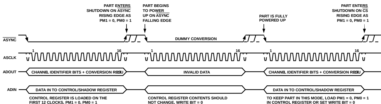
Figure 66. Autosutdown Mode Operation
