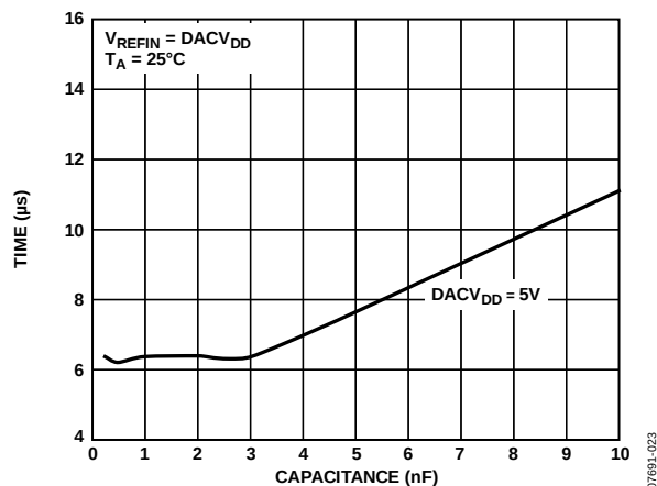
Figure 23. DAC Settling Time vs. Capacitive Load
