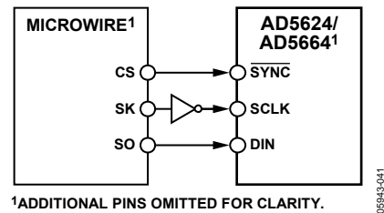
Figure 39. MICROWIRE Interface to AD5624/AD5664
