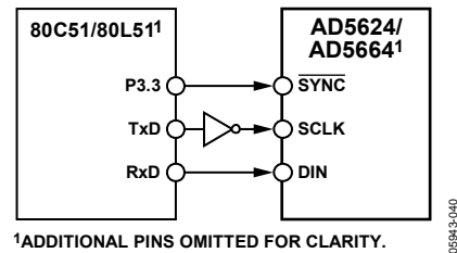
Figure 38. 80C51/80L51 Interface to AD5624/AD5664
