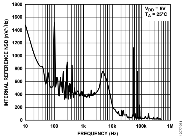
Figure 31. Internal Reference Noise Spectral Density vs. Frequency
