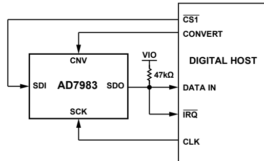
Figure 32. \overline{CS} Mode, 4-Wire with Busy Indicator Connection Diagram
