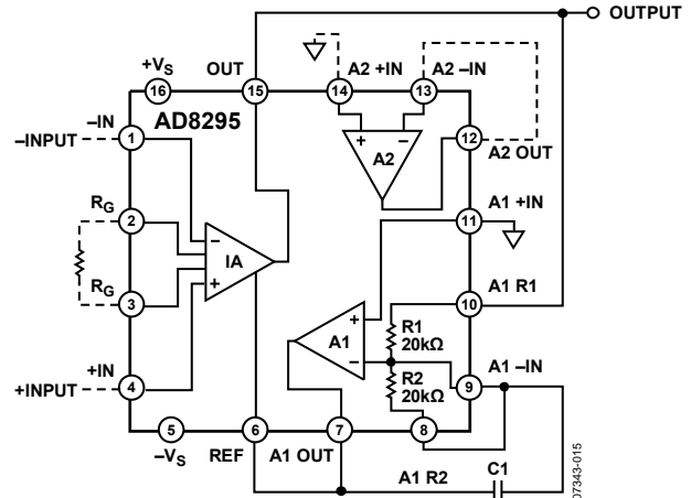
Figure 70. AC-Coupled Connection
