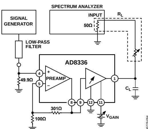
Figure 64. Harmonic Distortion
