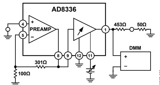
Figure 60. Offset Voltage
