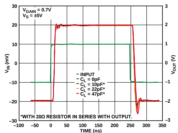
Figure 50. Large-Signal Pulse Response for Various Values of Load Capacitance Using \pm 5 V Power Supplies (See Figure 65)
