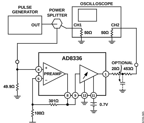
Figure 65. Pulse Response
