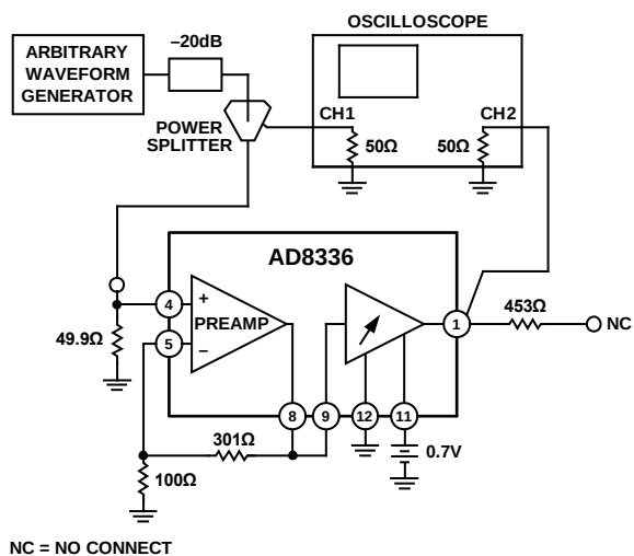
Figure 67. VGA Overdrive Recovery
