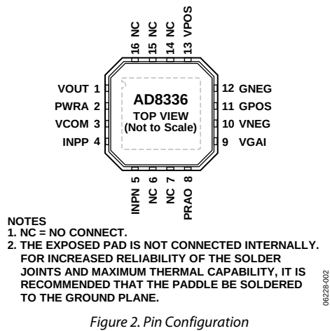
Figure 2. Pin Configuration
