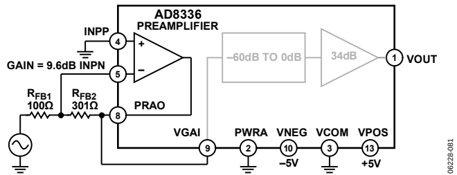
Figure 81. Circuit Configuration for Inverting Gain
