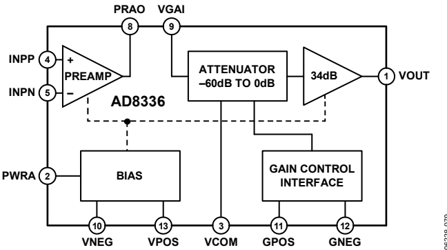
Figure 79. Application Block Diagram
