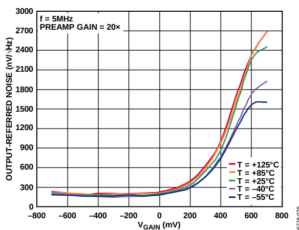
Figure 29. Output-Referred Noise vs. V_{GAIN} at Various Temperatures ( T ) When the Preamplifier Gain is 20\times (See Figure 62)
