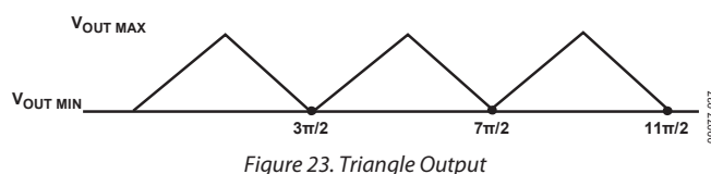
Figure 23. Triangle Output
