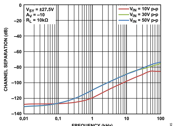
Figure 47. Channel Separation vs. Frequency, V_{SY} = \pm 27.5\text{ V}
