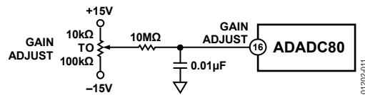
Figure 11. Gain Adjustment Circuit
