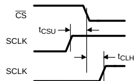
Figure 5. SCLK and \overline{\text{CS}} Timing Parameters
