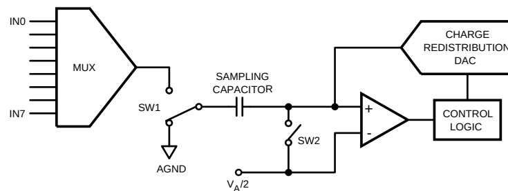
Figure 36. ADC088S102 in Hold Mode
