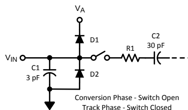
Figure 38. Equivalent Input Circuit
