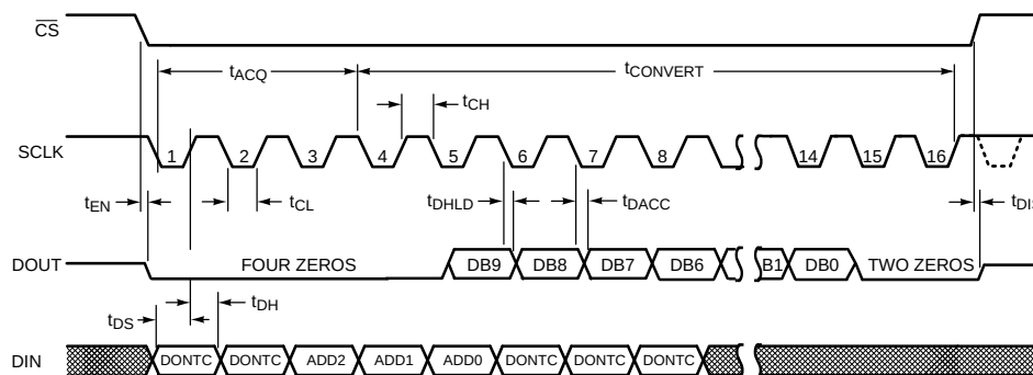
Figure 3. ADC088S102 Serial Timing Diagram
