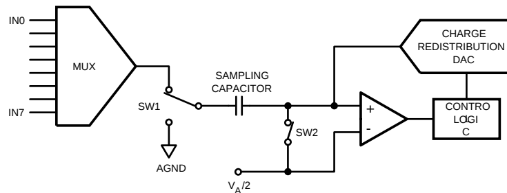
Figure 35. ADC088S102 in Track Mode
