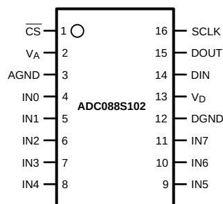
Figure 1. 16-Lead TSSOP See Package Number PW0016A
