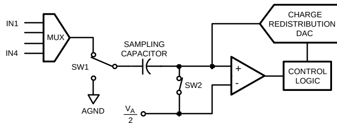
Figure 48. ADC104S101 in Track Mode
