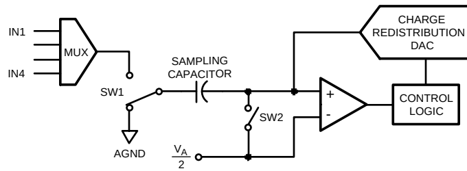
Figure 49. ADC104S101 in Hold Mode
