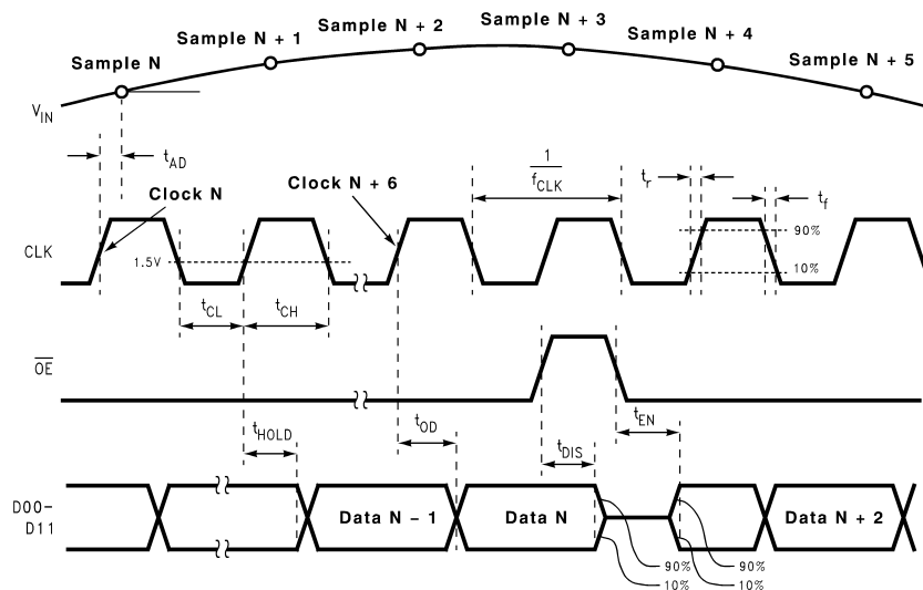
Figure 3. Output Timing
